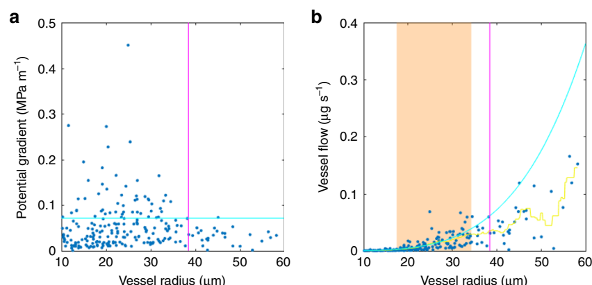
Fig. 7 The relationship between vessel radius, pressure gradient and flow rate. For all vessels in the inner region, with radius over 10 \mu\text{m} ( n = 306 ), the gradient ( a ) and flow rate ( b ) are shown as a function of lumen radius. In a , the magenta line shows flow-weighted mean vessel radius and the cyan line shows flow-weighted mean gradient. In b , the magenta line shows flow-weighted mean vessel radius, the cyan curve shows idealized (Hagen-Poiseuille) flow rate over the range of radii 10–60 \mu\text{m} for the flow-weighted mean gradient, orange zone shows the range of radii over which the idealized relationship fits the flow-radius points (t-test of residuals from points in 6- \mu\text{m} window cannot reject 0 mean at \alpha = 0.05 ; p -values, t -statistics, and degree of freedom counts of separate tests in Supplementary Table 1), and yellow curve shows the running mean flow rate over a 6- \mu\text{m} window.
