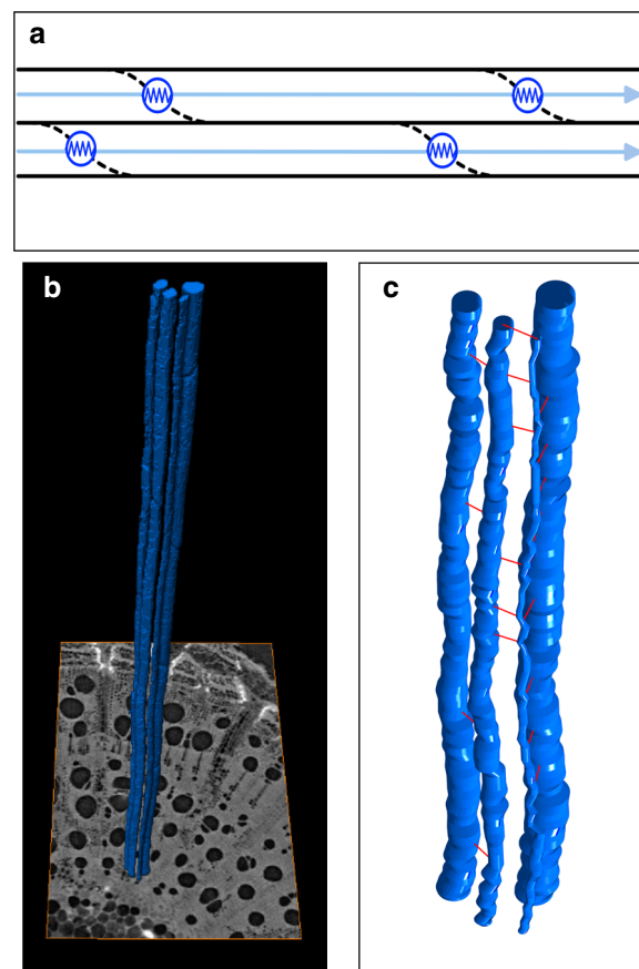
Fig. 1 Idealizations of xylem anatomy vs. networks derived from X-ray micro-computed tomography (μCT). a Current working model of xylem simplifies the xylem to parallel files of conduits of equal length, allowing it to be subdivided into units of one lumen and one end-wall resistance. Successive lumina are connected serially, with no connections across vessel files. b Four vessels (blue) segmented from a 3D stack of μCT images (at base). c Idealization of the same four vessels in the present model: each lumen is represented as circular in cross-section, with radius deduced from the data; connections (red) are placed at the centre of intervals where images show vessels to be connected.
