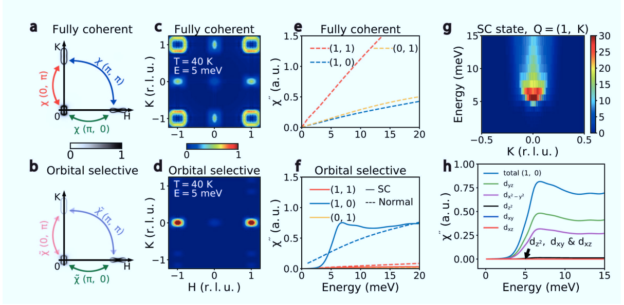
FIG. 5: Theoretical calculations of the spin fluctuations in detwinned FeSe. Map of the spectral function at zero energy for our model of the electronic structure of FeSe in (a) the fully coherent case with quasiparticle weights ( Z_\ell = 1 ) and (b) the orbital-selective case where reduced quasiparticle weights ( Z_\ell < 1 ) weaken the spin-fluctuations at certain momentum transfer (blue and red arrows) while the spin fluctuations stemming mostly from the d_{yz} orbital become dominant (green arrow). (c) For the fully coherent model, one obtains in the normal state large contributions to the dynamical structure factor close to (\pm 1, \pm 1) from the d_{xy} orbital and an almost identical but weaker contribution at (\pm 1, 0) and (0, \pm 1) . (e) The susceptibility integrated around these momentum transfer vectors, shows the same trend at low energies. (d,f) In contrast, the orbital selective model yields spin fluctuations at low energies which are dominated by peaks at (\pm 1, 0) in the low energy range shown. The enhancement of the spin fluctuations at (\pm 1, 0) in the superconducting state is clearly seen when plotted (f) as function of energy and (g) as an intensity map in momentum-energy space. (h) The spin fluctuations at (1, 0) are dominated by the contributions of the d_{yz} orbital.
