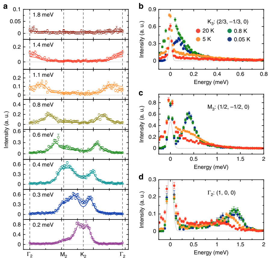
Fig. 4 Constant energy cuts along the high-symmetry directions and constant Q cuts at the high-symmetry points. a Constant energy cuts along the \Gamma -M-K- \Gamma direction at the indicated energy at 0.05 K. The solid curves indicate the simulated spin excitations using the model specified in the text and the vertical dashed lines indicate the high-symmetry points. b-d Constant Q cuts at the K, M and \Gamma points at various temperatures. The data presented in a , c and d were measured with E_i = 4.8 meV while the data in b were measured with E_i = 1.7 meV. The gray dashed lines indicate the elastic incoherent scattering. The error bars indicate the standard deviation
