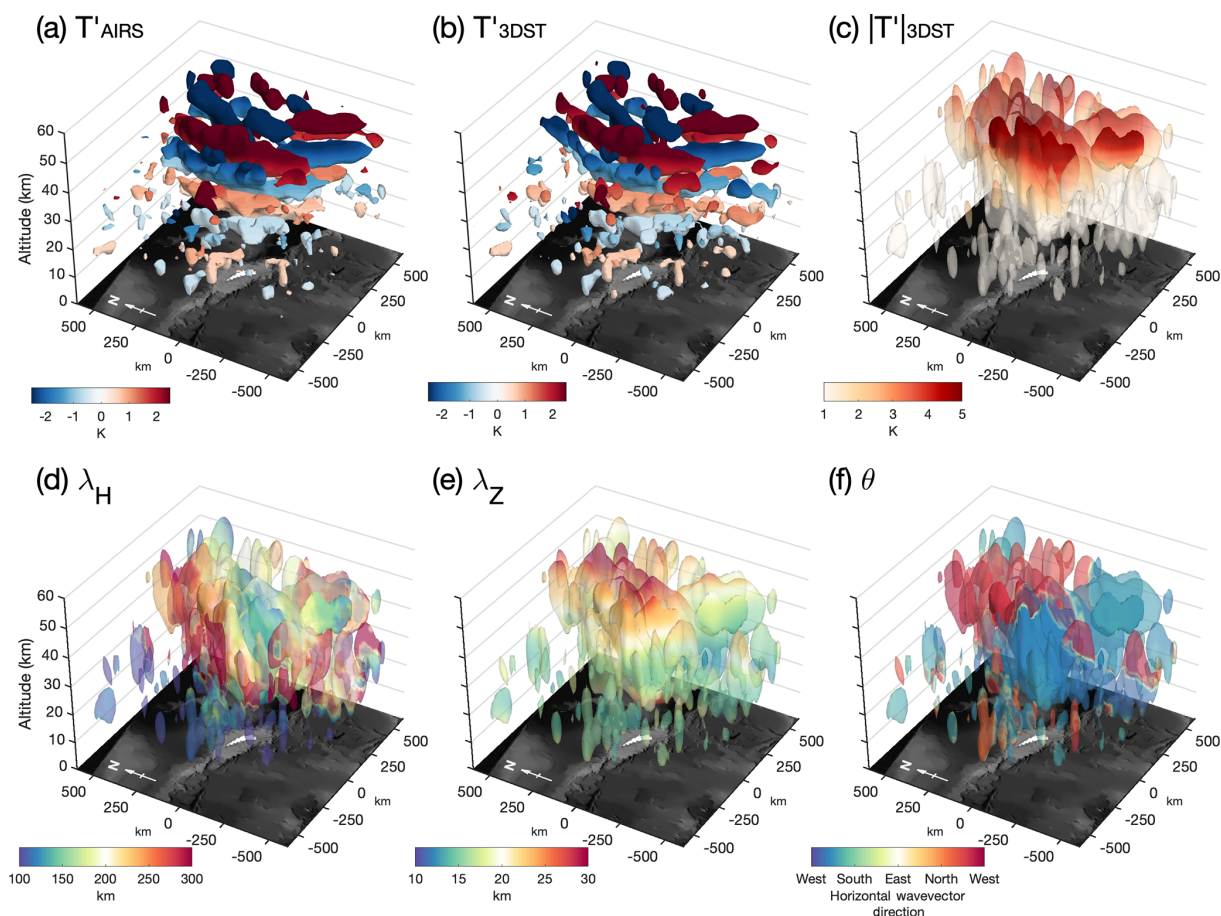
Figure 5. As Fig. 4, but for 3DST analysis of 3-D AIRS temperature measurements over the island of South Georgia ( 54^\circ S, 36^\circ W) on 5 July 2010 (granule numbers 034–035). For details, see text in Sect. 4.2.
