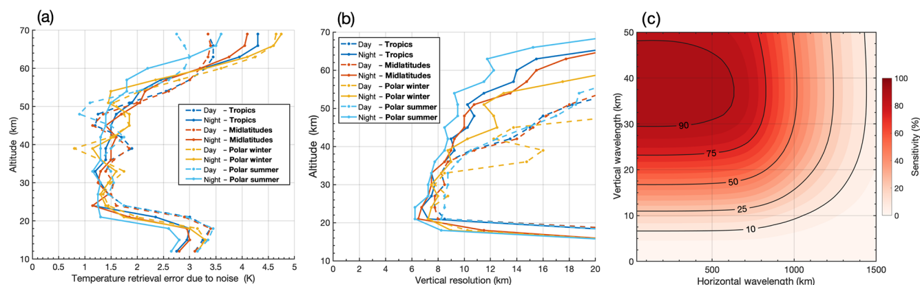
Figure 2. Estimated temperature retrieval errors (a) and vertical resolutions (b) for the 3-D AIRS temperature measurements against altitude for different atmospheric conditions, based on latitude and season. Dashed and solid lines indicate the daytime and nighttime retrievals respectively. Panel (c) shows estimated sensitivity of the detrended 3-D AIRS temperature perturbations to waves with different vertical and horizontal (across-track) wavelengths for observations made under average atmospheric conditions at an altitude of z = 40 km. For details, see text in Sect. 2.2.
