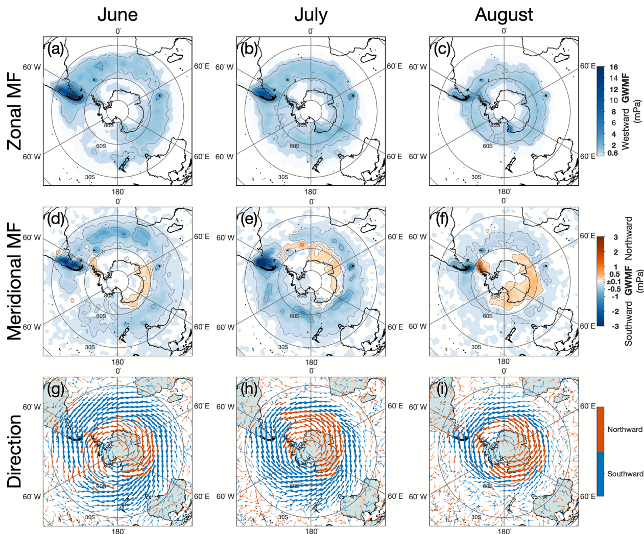
Figure 8. Monthly mean zonal (a, b, c) and meridional (d, e, f) gravity wave momentum flux at z = 40 km during June, July and August 2010. Monthly mean northward (southward) horizontal wavevector directions (g, h, i) are shown by orange (blue) arrows. The thicknesses of the arrows in (g, h, i) are scaled for mean wave amplitude in the corresponding months from Fig. 7a–c.
