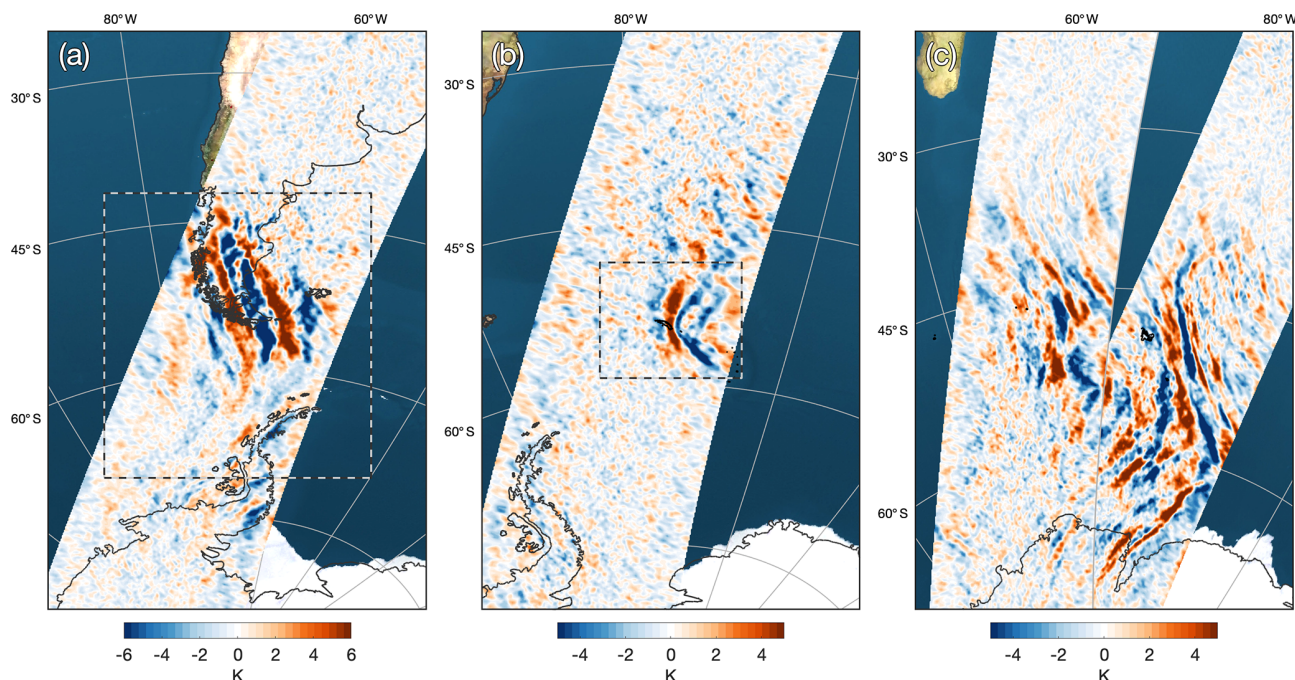
Figure 1. Temperature perturbation measurements along the AIRS scan track at an altitude of z = 40 km during overpasses on (a) 1 June over South America and Antarctic Peninsula, (b) 5 July over the island of South Georgia and (c) 28 June 2010 over the Southern Ocean. Panel (c) shows two consecutive overpasses on the same day. This is one vertical layer in a 3-D volume of AIRS temperature measurements between altitudes of 20 km and 60 km, using the retrieval of Hoffmann and Alexander (2009). Dashed lines in (a) and (b) indicate the regions considered in the 3-D case studies in Figs. 4 and 5.
