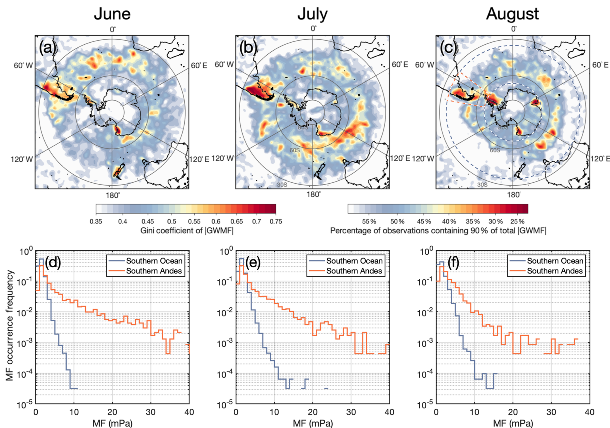
Figure 9. Panels (a, b, c) show the Gini coefficient of absolute gravity wave momentum flux (GWMF) for each month of AIRS measurements at z = 40 km for June, July and August 2010. One colour bar shows the value of the Gini coefficient, while the other shows the corresponding fraction of wave events attributable to 90 % of the total monthly absolute GWMF. The same colour scale and limits are used such that both properties directly correspond. Orange and grey dashed lines in (c) show regions defined over the southern Andes and Southern Ocean, as used in Table 2. Probability density functions (PDFs) of GWMF at z = 40 km over these regions for the corresponding months are shown in panels (d, e, f).
