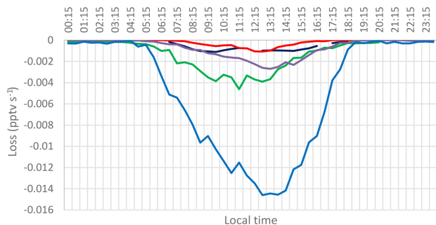
Figure 5. Photochemical production and loss of \text{H}_2\text{O}_2 in \text{pptv s}^{-1} . Note that the time used is local time.
