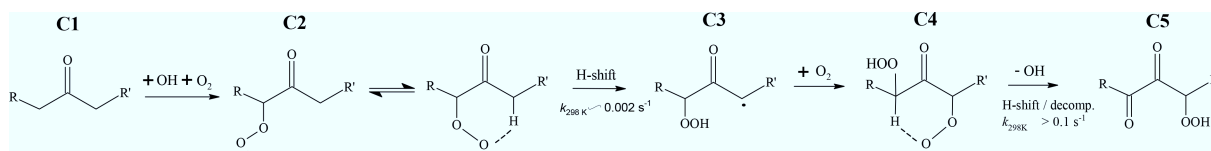
Figure 1. Autoxidation in OH-initiated oxidation of ketones. Following reaction with OH, the ketone C_1 forms a peroxy radical ( C_2 ) which undergoes an H-shift isomerization to form a hydroperoxide with a radical center on the carbon atom from which the hydrogen atom was abstracted ( C_3 ). Subsequent rapid addition of O_2 forms a new RO_2 radical ( C_4 ), which undergoes another H-shift, in this case terminating the autoxidation process by loss of an OH radical, resulting in a dicarbonyl hydroperoxide. In this scheme, the steps between C_2 and C_4 define the autoxidation. Adapted with permission from ref 6. Copyright 2013 American Chemical Society.
