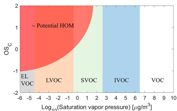
Figure 4. Relation between HOM and volatility classes in C*–OS C space. In this space, the volatility classes are well-defined, but the position of potential HOM will again depend on the exact functionality of the molecules. This C*–OS C space is discussed in more detail in section 5.1.
