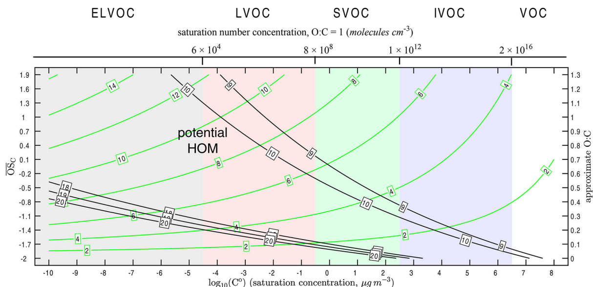
Figure 10. HOM saturation concentration ( C^* ), average carbon oxidation state ( OS_C ), and average O:C. Solid black lines extending from upper left to lower right are average carbon number ( n_C ). Solid green curves bending from top to lower left are average oxygen number ( n_O ). The broad volatility classes are indicated along the top, with corresponding colors in the figure; the number concentrations of compounds with O:C = 1 for the boundaries between these classes are indicated on the secondary x axis.
