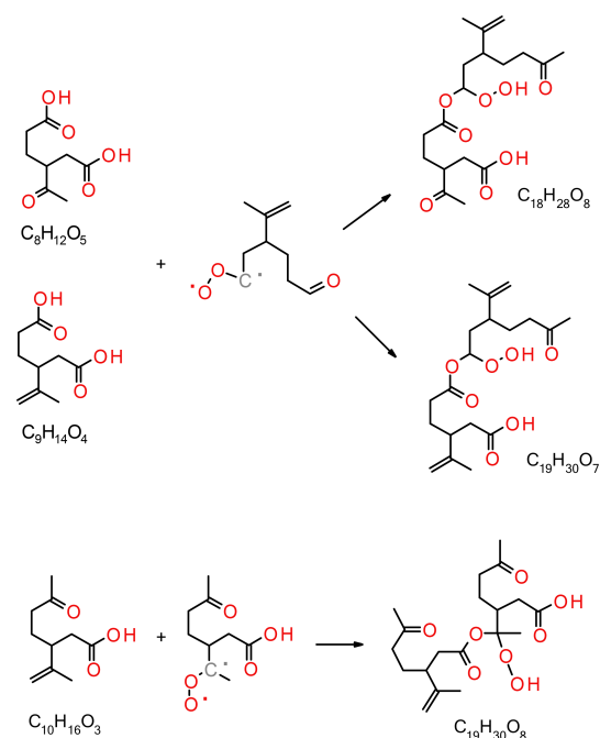
Figure 7. Proposed formation of observed dimers (C 18 H 28 O 8 , C 19 H 30 O 7 and C 19 H 30 O 8 ) from monomer–Criegee reactions.
