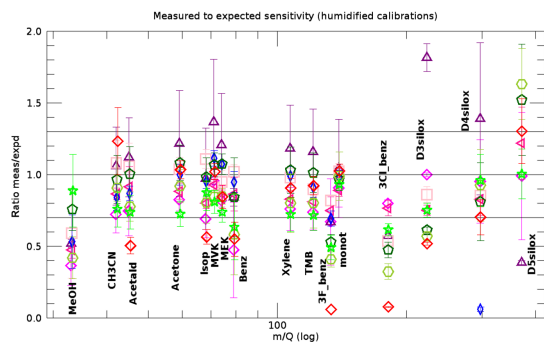
Figure 7. Measured versus expected sensitivities retrieved from humidified injections for all compounds in the gas standard and all PTR-MS instruments. The error bars represent the standard deviation of all gas standard injections with humidified \text{N}_2 or air as carrier gas. Compounds as in Fig. 4.
