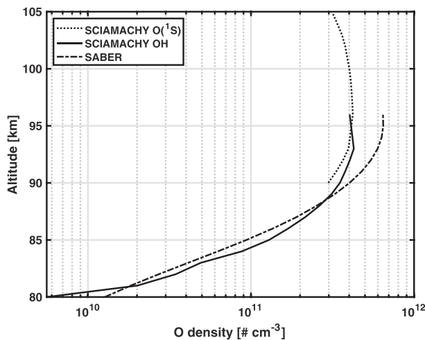
Figure 1. Global mean atomic oxygen density profiles from SCIAMACHY O( 1 S) (dotted, Kaufmann et al., 2014), SCIAMACHY OH (solid, Zhu & Kaufmann, 2018), and SABER (dash dotted, Mlynczak et al., 2018) and S18).
