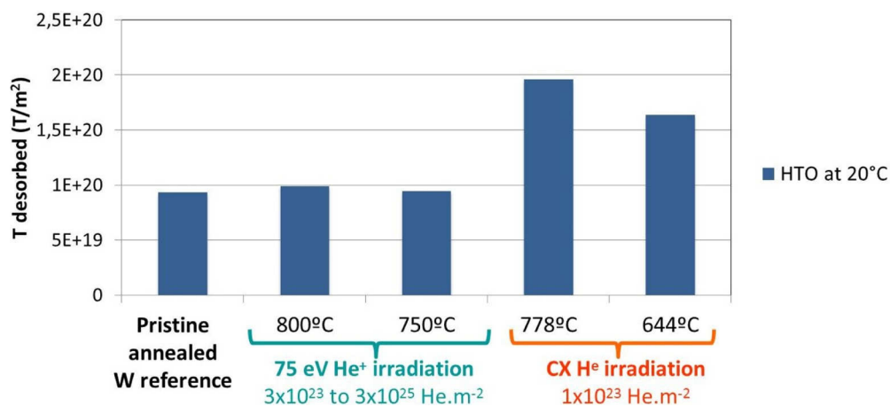
Fig. 8. T inventory desorbed as HTO at room temperature varies strongly depending on the irradiation type: 75 eV \text{He}^+ samples have a similar inventory than the pristine Wref, but in spite of the lower He fluence the CX He samples have significantly larger inventories.
