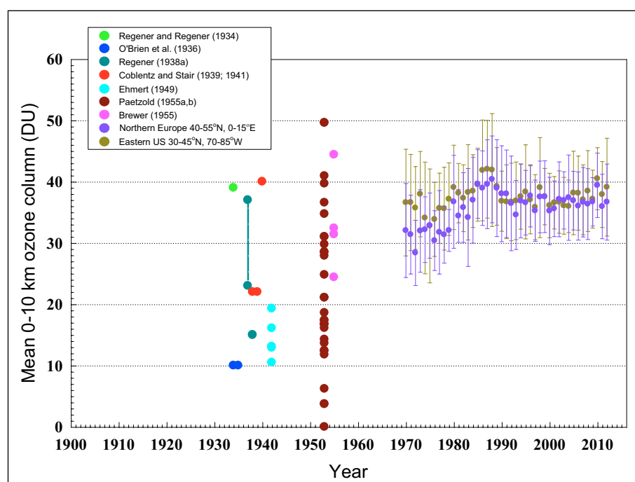
Figure 7: Historical measurements of free tropospheric ozone. Values shown are integrated 0–10 km ozone amounts. The difference between the ascent and descent of 30 October 1937 (dashed line) is probably an indication of the uncertainty of the differencing method, since it is unlikely that ozone changed by that much in less than a day. The modern values shown are annual averages for the 15^{\circ} \times 15^{\circ} regions around the locations of most of the historical ascents (northern Europe and the eastern US), calculated from ozonesondes using the TOST product (Section 4.4). The error bars indicate standard deviations of the monthly averages (atmospheric variability), not uncertainty of the measurement. DOI: https://doi.org/10.1525/elementa.376.f7
