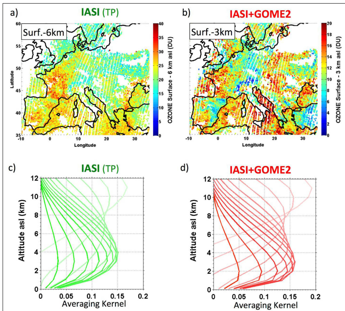
Figure 22: Satellite retrieval of ozone on 19 August 2009 over Europe (a) in the lower troposphere (up to 6 km asl) derived from the IASI Tikhonov-Philips approach (Eremenko et al., 2008) and (b) in the lowermost troposphere (up to 3 km asl) from the IASI+GOME2 multispectral synergism (Cuesta et al., 2013). Examples of averaging kernels in the troposphere for a satellite pixel over land for (c) IASI (TP) and (d) IASI+GOME2. DOI: https://doi.org/10.1525/elementa.376.f22
