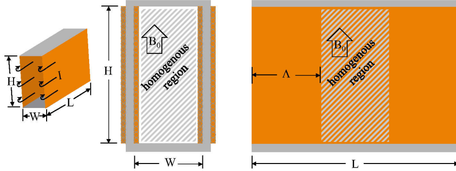
Figure 1. A diagram of an idealized magic box. The geometry is a perfect rectangular tunnel of \mu -metal and the \mu -metal has very high, and non-saturating permeability. The coils on either side (orange) are wrapped around the \mu -metal and are perfectly uniform current sheets that extend from the bottom to top of the sides. The direction of the current, I in the current sheets is indicated with the arrows in the left hand side diagram.
