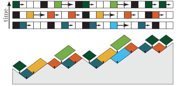
FIG. 2. Mapping the NaSch dynamics ( v_{\text{max}} = 2 , p = 0.25 ) to a KPZ-like surface growth. The upper half shows a NaSch configuration evolving in time and the lower half the corresponding height profiles. Vehicles are color coded and the arrows indicate their velocities determined by update step 3. The colors of the vehicles/diamonds are guides for the eye helping to distinguish increasing time (blue \rightarrow orange \rightarrow green) and velocities (dark \rightarrow light). White sites correspond to empty sites. Mapping a vehicle to a down-slope ( \blacksquare \rightarrow \searrow ) and an empty site to an up-slope ( \square \rightarrow \nearrow ), one translates a configuration at fixed time to a height profile. If a vehicle moves to the right, then according to the update rules a diamond of velocity size is added to the surface between the initial and final position.
