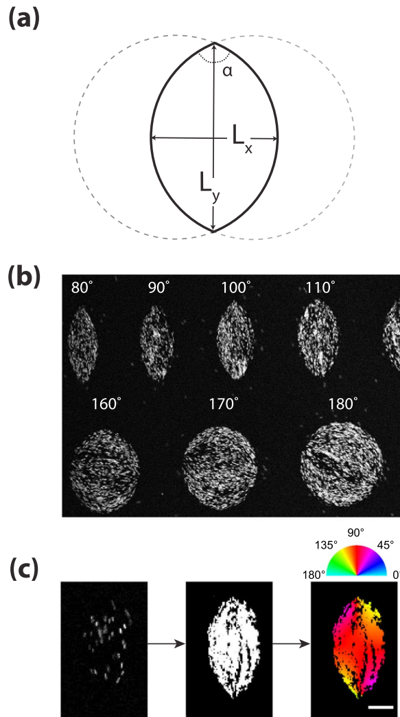
Figure 1. (a) Schematic of the tactoid geometry. (b) Subset of the experimentally employed wells organized according to their opening angle \alpha ( L_y = 30\mu\text{m} , maximum intensity projection image). (c) From left to right: Example of experimental image (single frame), maximum intensity projection of all frames collected for the same well, and image obtained after orientational analysis (scale bar 5\mu\text{m} ).
