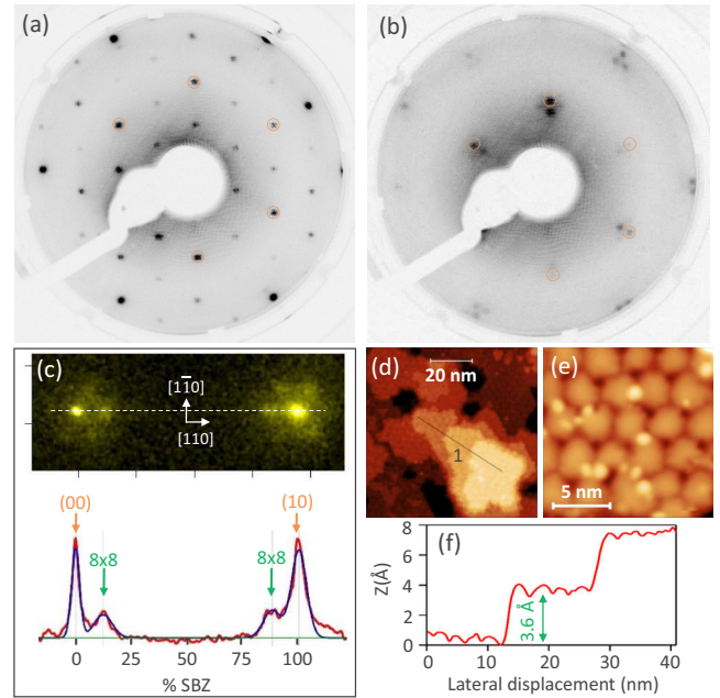
FIG. 1. (a) LEED taken at E = 45 eV on a clean InSb(111)A substrate exhibits 2 \times 2 surface reconstruction [orange circles denote 1 \times 1 spots]. (b) LEED taken at E = 45 eV on 10 nm-thick \alpha -Sn(111) film. Apart from the expected 1 \times 1 structure (orange circles), additional spots of high-order surface reconstruction are observed. (c) Spot-profile analysis LEED data taken at E = 87 eV and corresponding line profile (data plotted in red, four-peaks fit plotted in blue) through (00) and (10) spots allow us to assign the new surface reconstruction to be 8 \times 8 . (d) STM data measured with U = 2 V, I = 50 pA at T = 4 K. (e) STM data on a smaller scale showing domains. (f) The height profile along the path labeled “1” in (d) reveals a step height of 3.6 \text{ \AA} .
