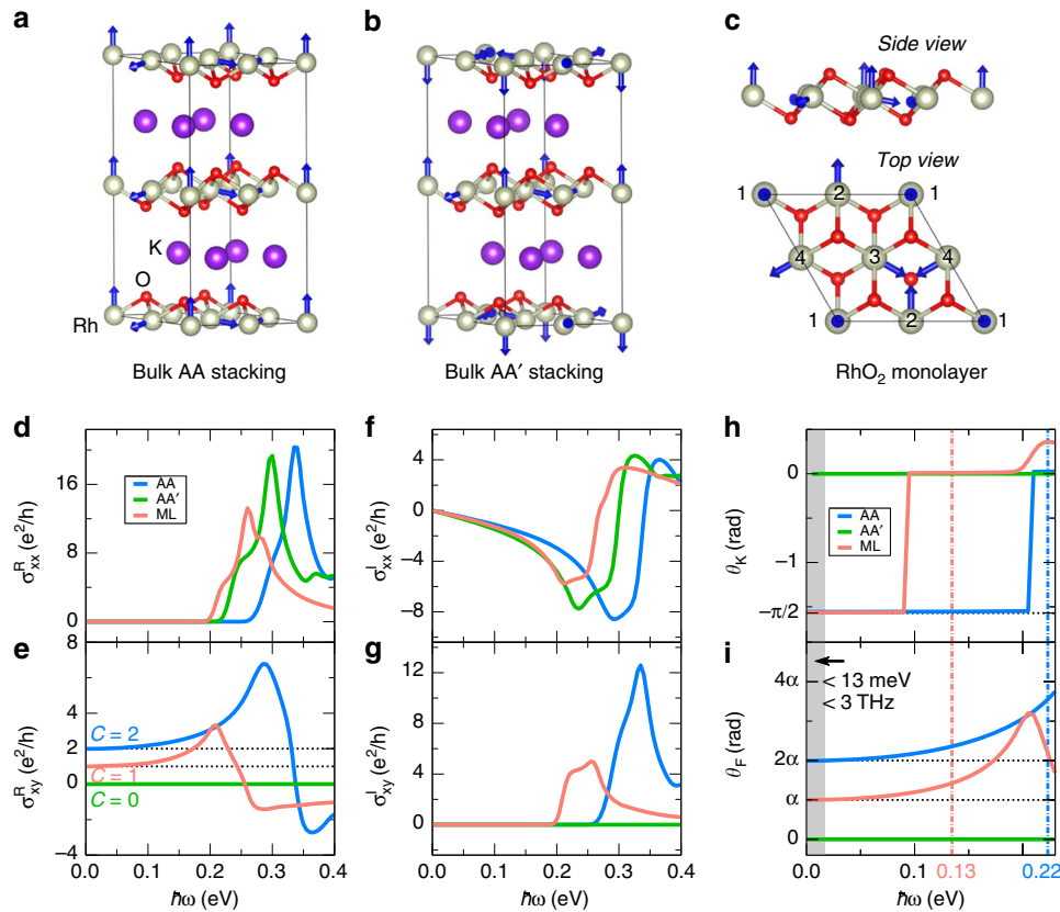
Fig. 4 Quantum topological magneto-optical effect in K_{0.5}RhO_2 . a, b Bulk AA and AA' stackings of K_{0.5}RhO_2 . c Side and top views of RhO_2 monolayer (ML). d–g The optical conductivities of K_{0.5}RhO_2 and RhO_2 ML. The results of K_{0.5}RhO_2 are scaled by the length of crystallographic z axis. For RhO_2 ML, the Fermi energy is moved upward to the topologically nontrivial band gap E_g (see Supplementary Fig. 5). h, i The Kerr and Faraday rotation angles of K_{0.5}RhO_2 and RhO_2 ML. The dash-dotted vertical lines indicate the E_g of the AA-stacked K_{0.5}RhO_2 (0.22 eV) and RhO_2 ML (0.13 eV). The shaded area marks the low-frequency limit (e.g., \hbar\omega < 0.1E_g^{ML} \approx 13 meV), in which the quantum topological magneto-optical effects can be measured by THz spectroscopy. Spin-orbit coupling is not included in d–i .
