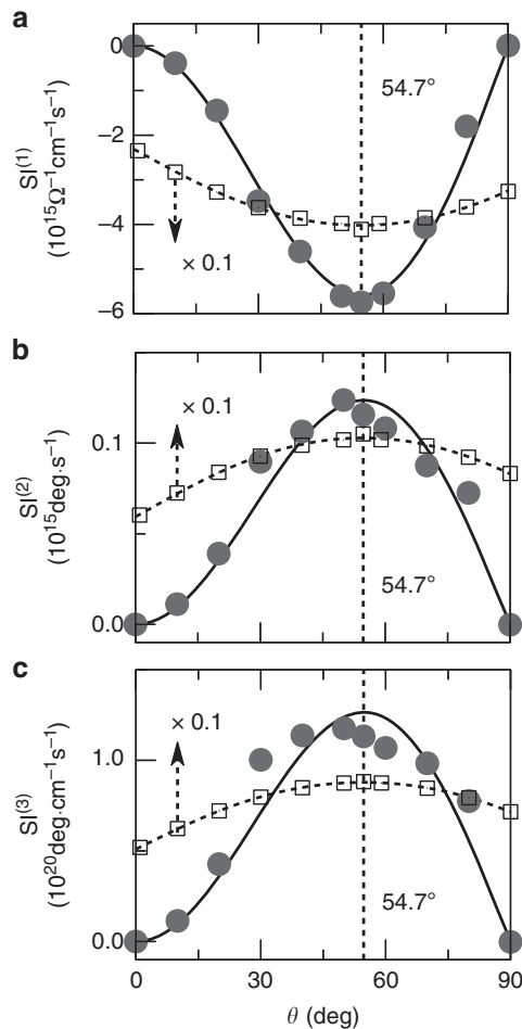
Fig. 5 Spectroscopic hallmarks of the topological magneto-optical effect.
