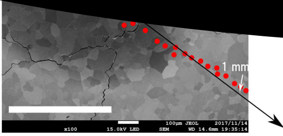
Fig. 1. SEM image of a sample after thermal shocks. This sample was exposed to He plasma at 1100 K. axis red points indicates observed grains for Fig. 5.
