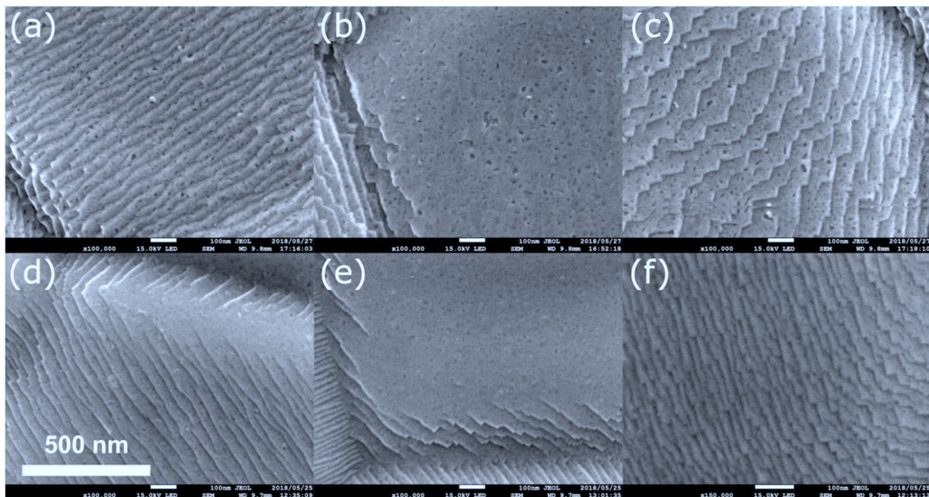
Fig. 2. SEM images of typical surface morphologies observed in the samples irradiated by He. (a), (b) and (c): taken from a sample irradiated at 470 K. (d), (e) and (f): taken from a sample irradiated at 1100 K.
