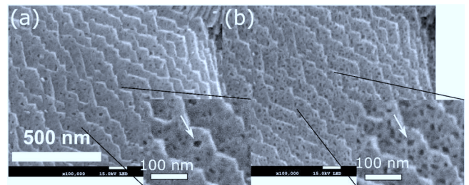
Fig. 6. Comparison between SEM images before (a) and after (b) the thermal shock experiment taken at the same position of a sample experienced He irradiation at 1100 K. This location belongs to the region b in the Fig. 5.
