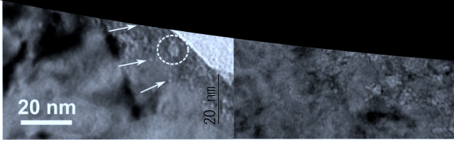
Fig. 3. Cross-sectional images observed by TEM of samples irradiated by He at (a) 470 K and (b) 1100 K.
