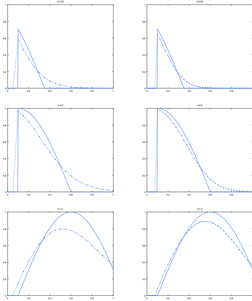
Figure 3: The columns show the numerical solutions (dashed lines) in comparison with the exact solution (continuous lines). The situations displayed in the right column are obtained using a grid twice as fine as in the left column.
