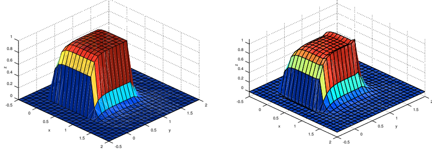
Figure 1: Numerical solutions of the linear two-dimensional problem after one time step with v = 1 (left) satisfying the monotonicity condition and with v = 1.5 (right), resulting in a monotonicity violation as in the one-dimensional case. The same behavior also occurs for velocities 1 < v < 1.5 , resulting in much less amplitudes of the violations.
