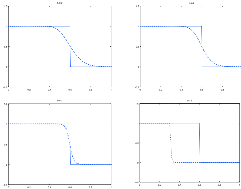
Figure 7: Numerical solutions (dashed lines) compared with the exact solution (continuous lines). The pictures correspond from left to right and top to bottom to the choices \mu = 1, 10, 100, 1000 .
