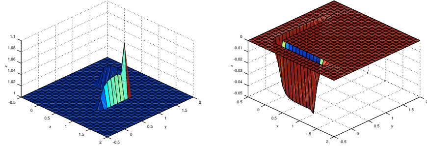
Figure 2: Plots showing in detail the monotonicity violation in the case \Delta t = \Delta x = \Delta y = 0.1 and v = 1.5 , obtained after one time step with the implicit Lax-Friedrichs scheme: The maximum of 1.0 and the numerical solution (left) and the minimum of 0.0 and the numerical solution (right).
