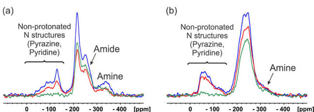
Figure 5. 15 N CPMAS NMR spectra of (a) Glu/Uro-1:4-250 and (b) Glu/Uro-1:0.17-250, obtained before and after deuterium exchange as a function of contact time. Blue: before deuterium exchange (contact time = 7000 μs); red: after deuterium exchange (contact time = 7000 μs); green: after deuterium exchange (contact time = 700 μs). The intensity of the spectra was normalized by using the mass of each sample.
