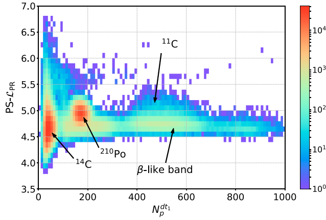
FIG. 4. Distribution of PS- \mathcal{L}_{\text{PR}} pulse-shape discriminator as a function of N_p^{dt_1} energy estimator. The plot is built using the entire set of data surviving the selection cuts described in Sec. II. The comparison with Fig. 3 allows to identify the range of values belonging to the \beta^- -like band indicated by the arrow.
