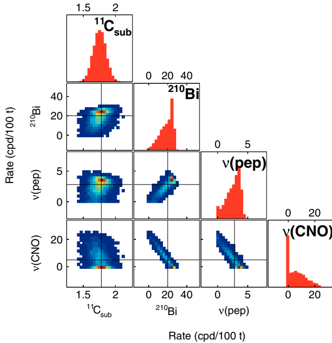
FIG. 6. This figure shows the results of the fit of MC simulated experiments obtained in the same conditions of Fig. 5 but, this time, removing all the constraints on R_{\text{CNO}} and R_{\text{pep}} . We only show here the correlation between \text{pep} , CNO, ^{11}\text{C} and ^{210}\text{Bi} , but the study included all the spectral components. The significant correlations among these species forbid to measure at the same time R_{\text{CNO}} and R_{\text{pep}} and to determine the ^{210}\text{Bi} decay rate. As described in the text, we have constrained the CNO rate to get the \text{pep} one and set a constraint on the ratio R_{pp}/R_{\text{pep}} to obtain a limit on the CNO flux.
