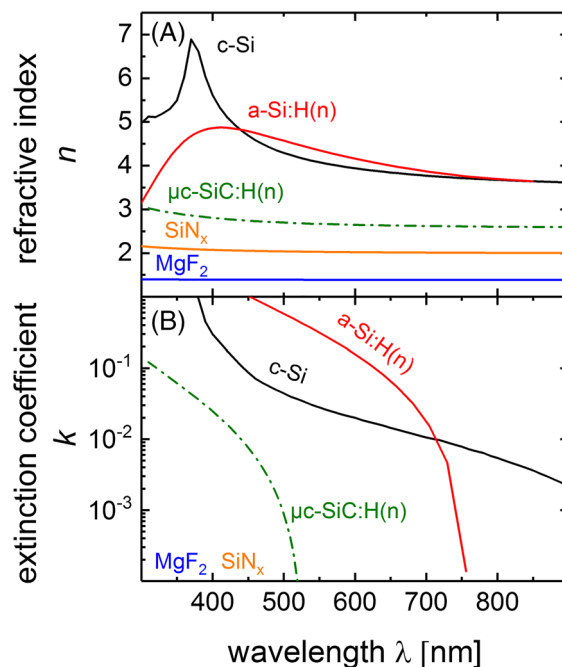
FIGURE 3 (A) Refractive index n and (B) extinction coefficient k derived from ellipsometry measurements of \mu\text{c-SiC:H(n)} , \text{SiN}_x , \text{MgF}_2 , \text{a-Si:H(n)} , 5 and c-Si. 21 The derived k is zero for \text{SiN}_x and \text{MgF}_2 . The full sets of n and k data for \mu\text{c-SiC:H(n)} , \text{SiN}_x , and \text{MgF}_2 can be found in the Supporting Information S1, S2 and S3 [Colour figure can be viewed at wileyonlinelibrary.com ]
