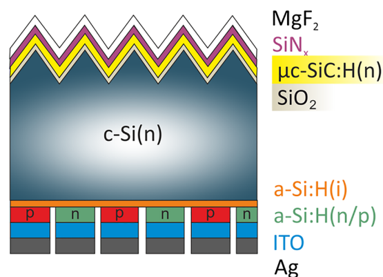
FIGURE 1 IBC c-Si solar cell with triple-layer ARC developed in this work. The triple-layer ARC consists of a 108 nm-thick MgF 2 layer, a 50- to 60 nm-thick SiN x layer, and a 0- to 60 nm-thick \mu c-SiC:H(n) layer. At the same time, the \mu c-SiC:H(n)/SiO 2 stack provides excellent surface passivation [Colour figure can be viewed at wileyonlinelibrary.com ]
