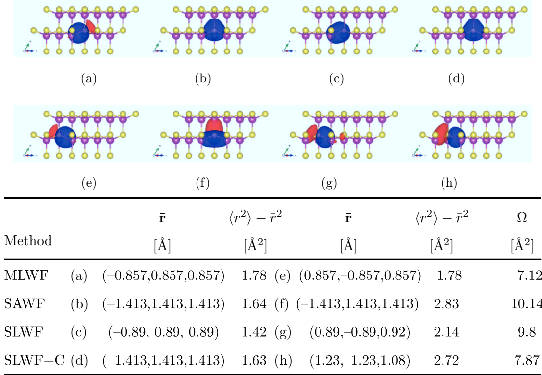
Figure 1. Top (figure): comparison of two representative Wannier functions resulting from different minimisation schemes for gallium arsenide (larger pink spheres: Ga cation atoms, smaller yellow spheres: As anions): (a), (e) MLWF; (b), (f) SAWF; (c), (g) SLWF; (d), (h) SLWF + C. For MLWF, SLWF and SLWF + C, four s -type orbitals centred at the midpoints of the four Ga–As bonds are used as the initial guess. In the case of SLWF and SLWF + C, we optimise the first WF (and also constrain its centre to sit at (\frac{1}{4}, \frac{1}{4}, \frac{1}{4}) , i.e. on the As atom, for SLWF + C), while all the other WFs are left unoptimised. For SAWF, one s -type and three p -type orbitals centred on the As atom are used as initial guess. Specifically, the first row shows one MLWF (a), one SAWF with s character centred on As (b), one WF obtained with the selective localisation scheme (c) and one WF obtained with the selective localisation scheme with additional constraints on its centre (d). The second row shows one of the other three WFs for all four methods. In particular: (e) MLWF, (f) SAWF with p character, (g) unoptimised SAWF and (h) unoptimised SAWF + C. For all plots we choose an isosurface level of \pm 0.5 \text{ \AA}^{-3} (blue for + values and red for – values) using the Vesta visualisation program [28]. Bottom (table): Cartesian coordinates of the centres \bar{\mathbf{r}} and minimised individual spreads \langle r^2 \rangle - \bar{r}^2 for the two representative Wannier functions of each of the four different minimisation schemes and initial guesses described above. We also report the total spread \Omega of all four valence WFs for each method.
