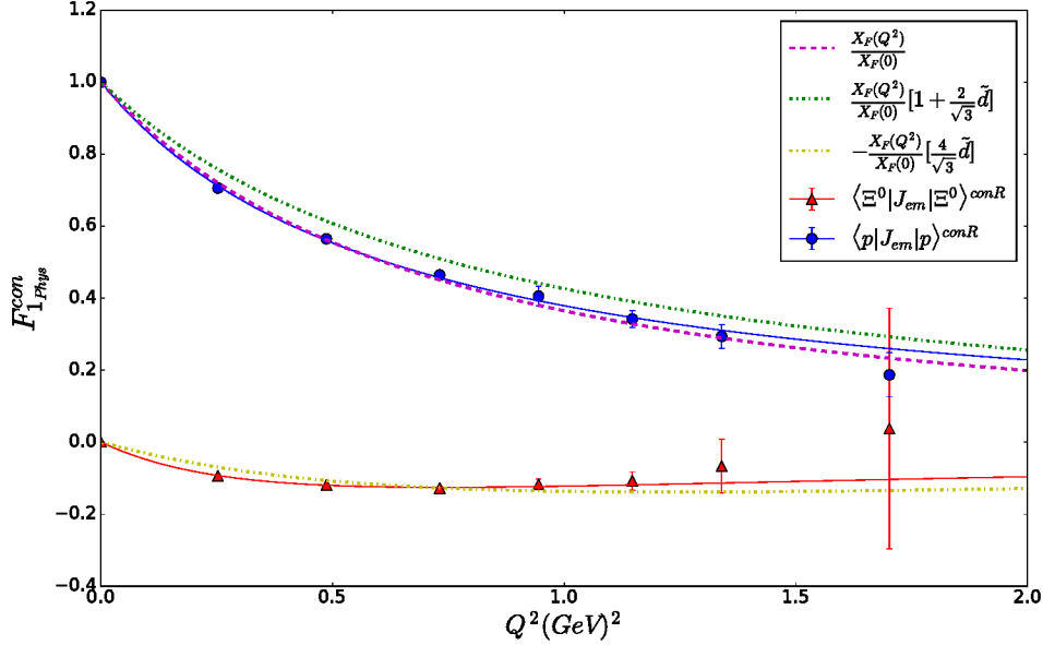
Figure 12: F_1^{\text{con R}} for the proton (filled circles) and \Xi^0 (filled triangles) at the physical point. The dashed line is X_F(Q^2)/X_F(0) . The dashed-dotted lines are the complete leading terms, for the proton: X_F(Q^2, \bar{m})/X_F(0, \bar{m})(1 + 2/\sqrt{3}\tilde{d}(Q^2, \bar{m})) and for \Xi^0 : X_F(Q^2, \bar{m})/X_F(0, \bar{m}) \times 4/\sqrt{3}\tilde{d}(Q^2, \bar{m}) , while the full lines are the complete expressions in eq. (119).
