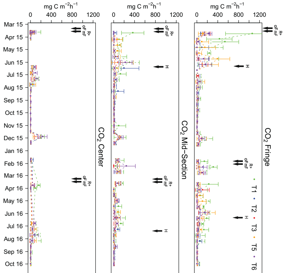
Figure 20: Seasonal variation of \text{CO}_2 fluxes, Ifakara, with indication of rice planting (R), organic fertilizer application (oF), mineral fertilizer application (mF) and harvest (H).
