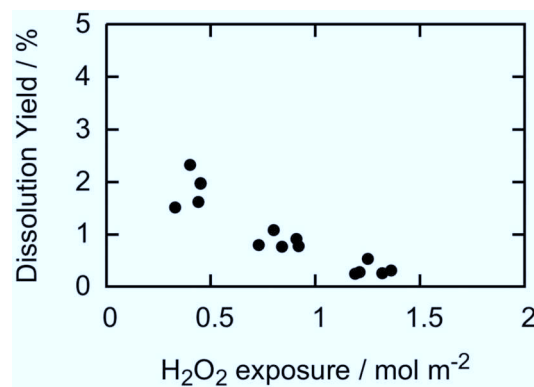
Fig. 2 Dissolution yield vs. accumulated H 2 O 2 consumption per m 2 of exposed UO 2 for pellets in this study.
