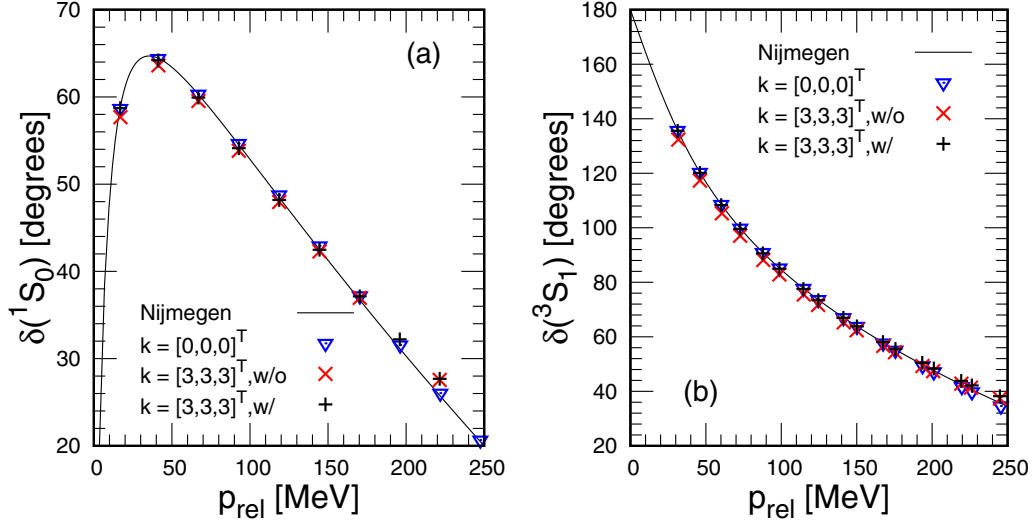
FIG. 4. S -wave neutron-proton scattering phase shifts calculated using the spherical wall method as a function of the relative momenta between the two nucleons.
