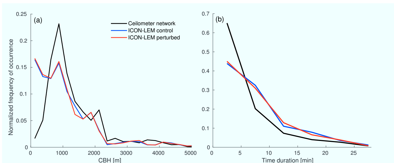
Figure 8. Left: Normalized cloud base height distribution (bin size: 250 m) of 51 ceilometer stations over Germany on 2 May 2013 (8 – 20 h UTC). Right: Normalized cloud lifetime (bin size: 5 min) for low-level clouds (<3 km) of few, scattered and broken cloud conditions (i.e. cloud cover between 5 and 87 %). Data from the DWD ceilometer network in Germany (black), and ICON-LEM C2R (blue) and P2R (red) simulations.
