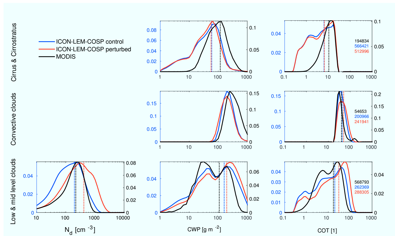
Figure 10. Probability distributions of droplet number concentration (left column, only for low, liquid clouds), cloud water path (liquid plus ice water, center column) and cloud optical thickness (right column) of Cirrus and Cirrostratus (top row), convective clouds (second row), and low and mid-level clouds (bottom row) from ICON-COSP simulator and MODIS (in total four overpasses on 2 May 2013). Left y-axis are for ICON-LEM-COSP and right y-axis for MODIS observations. Straight-dotted lines display means. The numbers on the right side show the number of pixels used for the PDF calculation.
