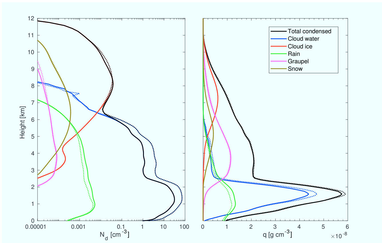
Figure 4. Vertical profile of (all-sky) domain mean number concentration (left) and mass concentration (right) of total water and individual particle species on 2 May 2013 from 8 h to 20 h UTC. The control (C2R) simulation is plotted as solid lines and the perturbed (P2R) simulation as dotted lines. Note the logarithmic x-axis for the number concentration panel. Hail not shown due to very low values.
