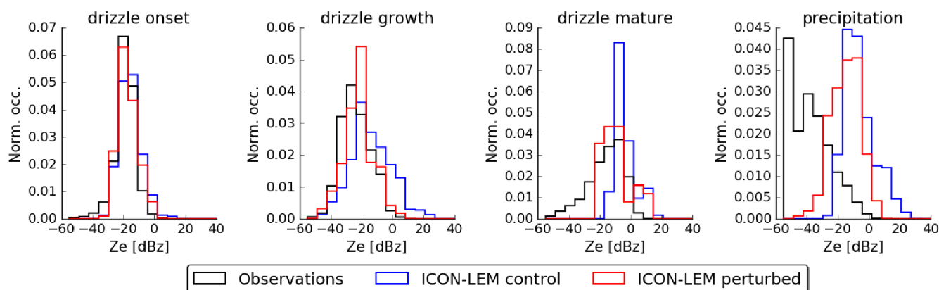
Figure 7. Normalized distributions for the different classes of drizzle development in Meteorological Observatory Lindenberg – Richard Abmann-Observatorium (MOL-RAO) on 2 May 2013. a) drizzle onset, corresponding to the small non-precipitating drizzle drops, larger than cloud droplets but not big enough to fall yet – this is only a signature in the skewness of the Doppler spectrum, not in reflectivity; b) drizzle growth, which contains the drops big enough to modify the spectra shape; c) drizzle mature, which is the drizzle precipitating inside the cloud; and d) precipitation, which is the class of precipitation below cloud base. The radar observations are processed as in Acquistapace et al. (2017), and ICON-LEM meteogram output at the MOL-RAO site is processed using the PAMTRA forward operator and processed analogously. Black: observations; blue: control simulation (C2R); red: perturbed simulation (P2R).
