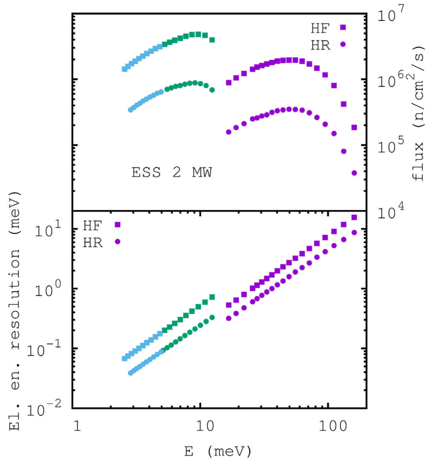
Fig. 32. Results of Vitess simulations of T-REX for flux and elastic energy resolution are shown as a function of incident energy at 2 MW ESS source power, for two anticipated chopper configurations termed HF (highest flux) and HR (highest resolution).
