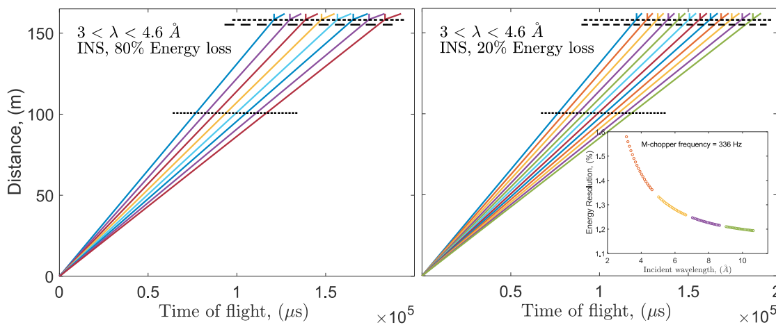
Fig. 30. Time of flight diagram for 3–4.6 Å neutrons across the 1.72 Å bandwidth of CSPEC. Dashed horizontal lines represent chopper positions and respective opening times. The coloured lines between the sample and detector indicate an energy loss of (left) 80% of E_i and (right) 20% of E_i , and an infinite energy gain. Inset: Range of elastic energy resolutions across the bandwidth for a range of incident wavelength settings with minimum wavelengths of: 3, 5, 7, and 9 Å.
