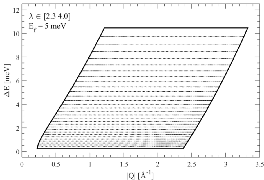
Fig. 35. Low angle continuous ( |Q| , E ) coverage of BIFROST for E_f = 5 meV in the wavelength interval 2.3–4 \text{\AA} , in high flux mode. The spacing between the horizontal dotted lines indicates the FWHM of the energy resolution of the primary spectrometer, at that energy transfer.
