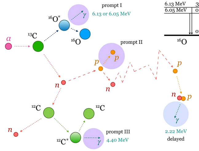
FIG. 22. Scheme of the (\alpha, n) interaction on ^{13}\text{C} . The three processes that can generate the three kinds of the prompt signals, prompt I , II , and III , as described in text, are shown in violet areas. The blue area indicates the delayed signal from the neutron capture.
