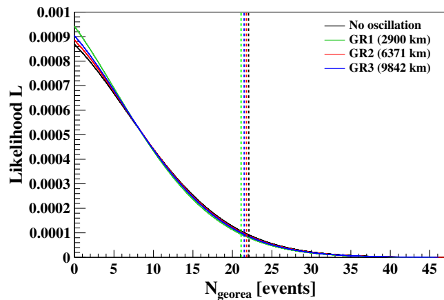
FIG. 57. Likelihood profiles for the number of georeactor events N_{\text{georeactor}} obtained in the spectral fits with the constrained number of reactor antineutrino events. The four profiles represent the fits that differ in the shape of the PDF used for the georeactor contribution (Fig. 34), corresponding to different source positions in the deep Earth [GR1, GR2, GR3, Fig. 21(a)] and to a no-oscillation hypothesis. The vertical dashed lines indicate the upper limit at 95% C.L. for N_{\text{georeactor}} as obtained in each of the four fits. In setting the upper limit on the power of the georeactor, that depends on the assumed location of the georeactor, we use conservatively the highest limit on N_{\text{georeactor}} equal to 21.7 events.
