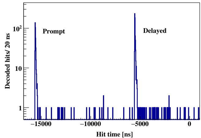
FIG. 26. Example of an IBD candidate, when both the prompt and the delayed are individual clusters in a single event of 16 \mu\text{s} DAQ time window. The negative hit times are expressed with respect to the trigger reference time.
