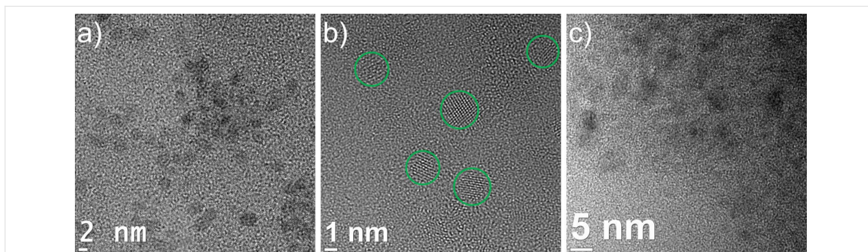
Figure 2: HRTEM images: a) Ni/Ga nanoparticles from a 1 wt % dispersion of \text{Ni}(\text{COD})_2 and \text{GaCp}^* in [\text{BMIm}][\text{BF}_4] after 24 h of dispersion and 10 min of microwave-induced decomposition. For details of the particle size distribution ( 2.5 \pm 0.5 nm), see Supporting Information File 1, Figure S2. b) Ni/Ga nanoparticles from 0.5 wt % dispersion of \text{Ni}(\text{COD})_2 and \text{GaCp}^* in [\text{BMIm}][\text{BF}_4] after 24 h of dispersion and 20 min of microwave-induced decomposition. For details of the particle size distribution ( 2.5 \pm 0.5 nm), see Supporting Information File 1, Figure S3. c) Ni/Ga nanoparticles from 0.5 wt % dispersion of \text{Ni}(\text{COD})_2 and \text{GaCp}^* in propylene carbonate after 24 h of dispersion and 20 min of microwave-induced decomposition. For details of the particle size distribution ( 5 \pm 1 nm), see Supporting Information File 1, Figure S4.
