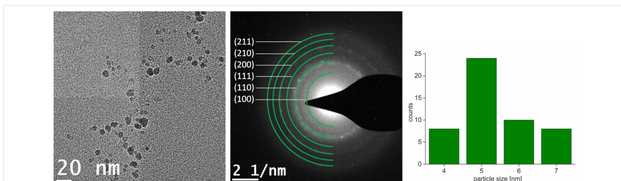
Figure 3: HRTEM image and particle size distribution of 0.5 wt % dispersion of NiGa nanoparticles from \text{Ni}(\text{COD})_2 and \text{GaCp}^* in [\text{BMIm}][\text{NTf}_2] after 24 h of dispersion and 30 min of microwave-induced decomposition. SAED with indexed reflections for NiGa (space group Pm\bar{3}m ). Particle size distribution 5 \pm 1 nm (50 particles counted).
