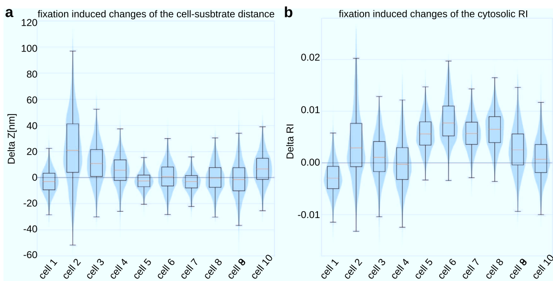
Figure 5. Fixation-induced changes in distance and refractive index. The changes in the cell–substrate distance and the cytosolic RI are evaluated for scanning point for 10 cells. a) We find prominent changes in the cell–substrate distance of cell 2 and cell 3 toward higher values while the remaining cells show random shifts. b) The cytosolic RI shows a systematic shift toward higher values after the fixation.
