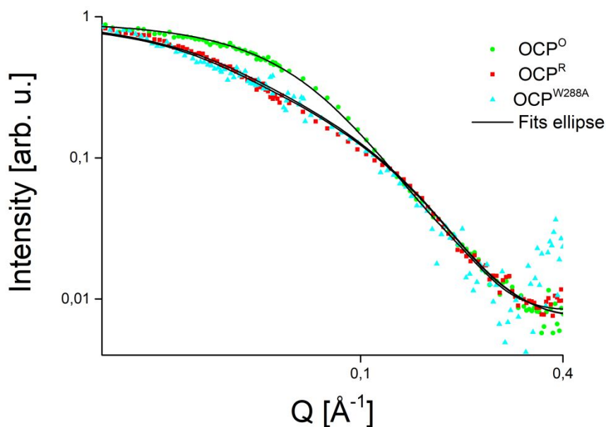
Figure 3: SANS data of OCP at a protein concentration of about 1 mg/ml obtained in the dark (green circles) and under constant illumination at 480 nm (red squares), respectively, measured at temperature of 15 °C using the instrument KWS-1. SANS data of OCP W288A measured under the same conditions are shown as cyan triangles. The black solid lines represent the fitting curves of the ellipsoid model (see Table 1).
