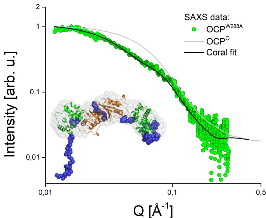
38 Figure 9: Verification of the solution structure of OCP W288A at a protein concentration of about 65 mg/ml 39 using SAXS data (green circles). The fit (black line) was obtained according to the CORAL structure of 40 OCP R shown in Figs. 5 and 6. For comparison, the grey line shows the fit function of OCP O shown in Fig. 5. 41 42 43 44
