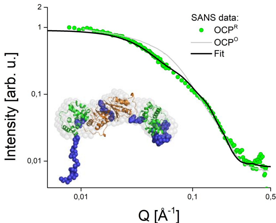
33 Figure 7: Analysis of SANS data of OCP under illumination at a protein concentration of about 1 mg/ml 34 measured at 15 °C (green dots): The fit (black line) corresponds to the reconstructed solution structure of 35 OCP R (depicted by grey spheres in the inset) obtained using the software package DAMMIN. The 36 corresponding dimeric structure obtained using CORAL below (see Fig. 9) and identified with OCP R is also 37 shown in the inset. Flexible areas in the OCP structure are indicated in blue, NTD and CTD are shown in 38 green and orange, respectively. For comparison, the grey line shows the SANS curve calculated for an 39 OCP O dimer, see Fig. 5. 40 41 42 43 44 45 46 47 48 49 50 51 52 53 54 55 56 57 58 59 60
