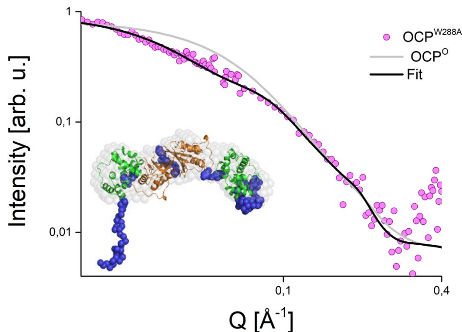
10 11 12 13 14 15 16 17 18 19 20 21 22 23 24 25 26 27 28 29 30 31 32 33 34 35 Figure 6: Analysis of SANS data of OCP W288A at a protein concentration of about 1 mg/ml measured at 36 15 °C (purple circles): The fit (black line) corresponds to the reconstructed solution structure of OCP W288A 37 (depicted by grey spheres in the inset) obtained using the software package DAMMIN. The corresponding 38 dimeric structure obtained using CORAL from SAXS data below (see Fig. 9) and identified with OCP R is 39 also shown in the inset. Flexible areas in the OCP structure are indicated in blue, NTD and CTD are shown 40 in green and orange, respectively. For comparison, the grey line shows the SANS curve calculated for an 41 OCP O dimer, see Fig. 5. 42 43 44 45 46 47 48 49
