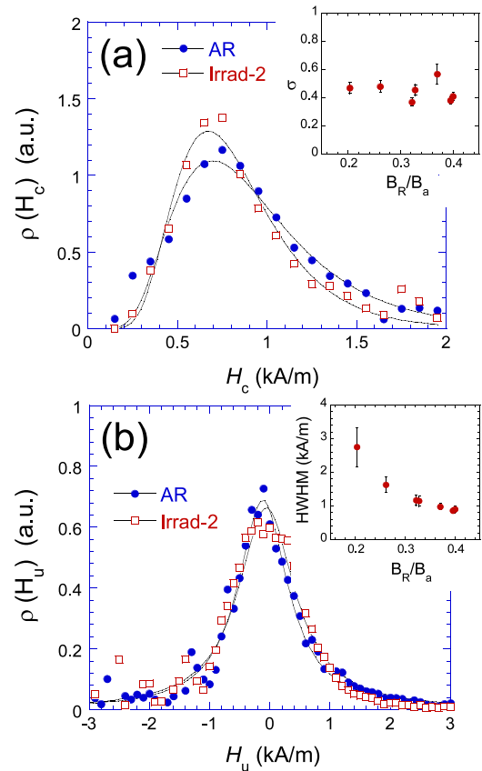
FIG. 2. FORC distribution curves along (a) H_c and (b) H_u axes, respectively, before and after neutron irradiation (Irrad-2). The data for VVER440 are shown as an example. The insets in (a) and (b) respectively show the width parameter \sigma and HWHM, as a function of B_r/B_a , obtained in different contact condition for the magnetic yoke and sample. Here, B_r and B_a are remanent and maximum flux densities of a major hysteresis loop, respectively.
