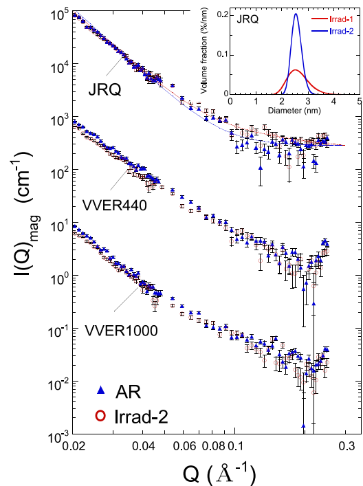
FIG. 4. Magnetic SANS intensities before and after neutron irradiation (Irrad-2). The data for JRQ and VVER440 are shifted upwards for clarity. The solid lines through the data for JRQ are least-squares fitting lines. The inset shows the volume distribution function of nanoscale features as a function of diameter after neutron irradiation for JRQ.
