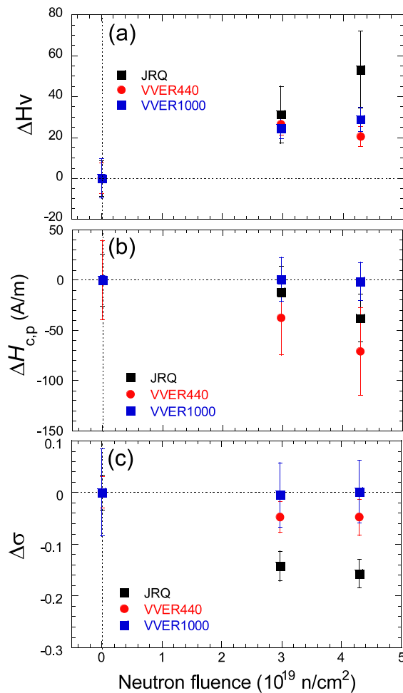
FIG. 3. Change of (a) hardness, (b) peak position and (c) width parameter of the FORC distribution peak along the H_c direction, as a function of neutron fluence.
