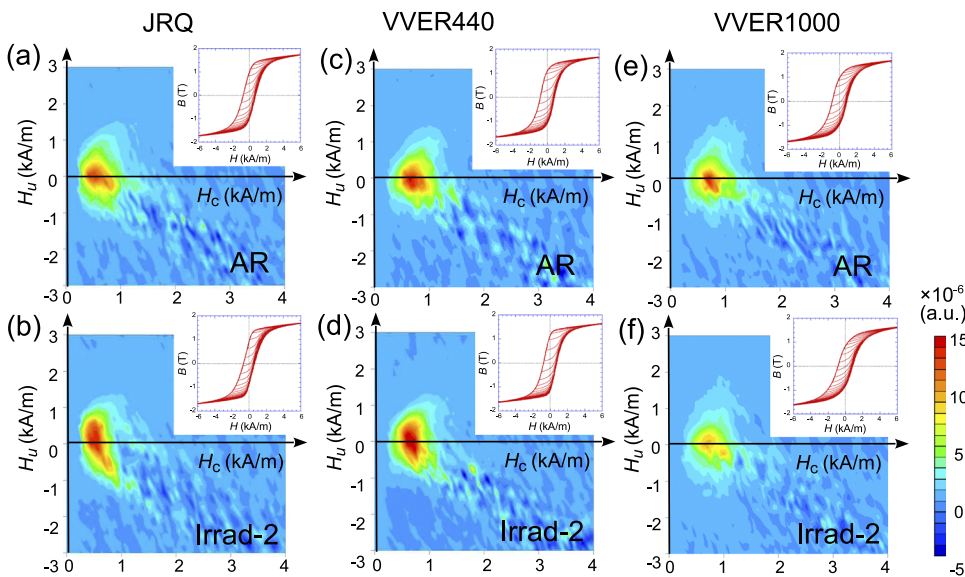
FIG. 1. FORC diagrams, taken before and after neutron irradiation (Irrad-2) for JRQ [(a), (b)], VVER440 [(c), (d)], and VVER1000 [(e), (f)]. The insets show measured FORCs, from which the FORC diagram was calculated.
