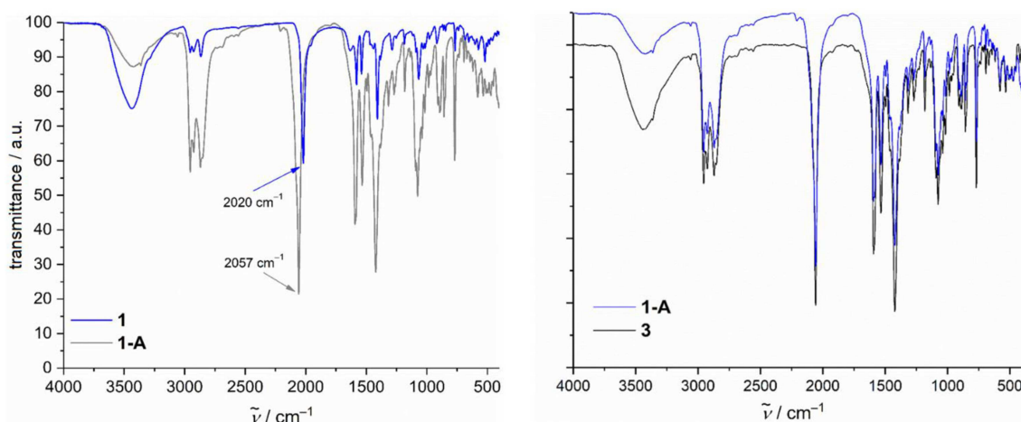
FIGURE 4 | Comparison of IR spectra of compounds 1 vs. 1-A (left) and 1-A vs. 3 (right).
