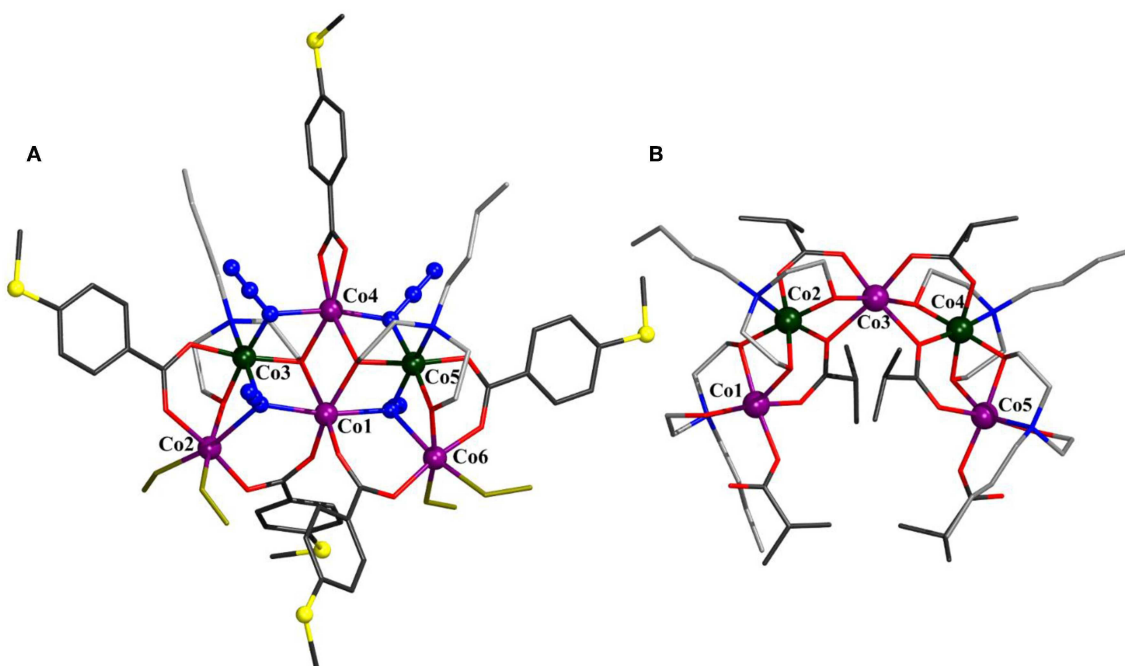
FIGURE 2 | Molecular structure of [\text{Co}^{\text{I}}\text{Co}^{\text{III}}(\text{N}_3)_4(\text{N-n-bda})_2(\text{bza-SMe})_5(\text{MeOH})_4]^+ in 2 ( A ) and comparison to [\text{Co}^{\text{I}}\text{Co}^{\text{III}}(\text{N-n-bda})_2(\text{N-n-Hbda})_2(\text{lb})_6] (Schmitz et al., 2016a) ( B ). Hydrogen atoms, Cl - counterion, and co-crystallized solvent molecules are omitted for clarity. The cobalt, sulfur, and the nitrogen atoms of azides are represented as ball-and-stick models. Color code: C (carboxylates) = dark gray; C (N-n-Hbda - and N-n-bda 2- ) = gray; N = blue; O = red; S = yellow; coordinated MeOH molecules = yellow sticks; Co I = violet; Co III = dark green. See Supporting Information for detailed crystal packing of the complexes.
