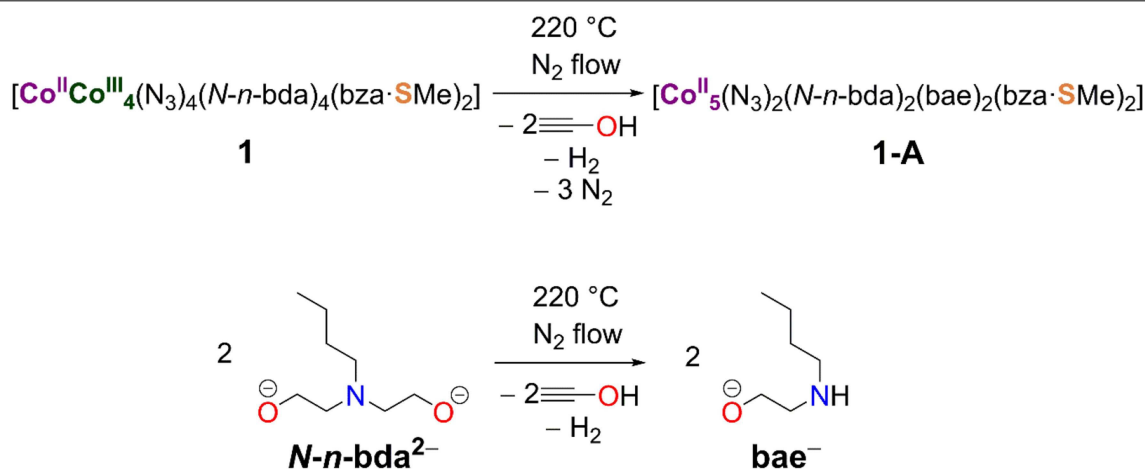
SCHEME 2 | Structural redox transformation of compound 1 to compound 1-A accompanied by the release of two azide groups and the conversion of the N - n -bda 2- ligand to bae - .
