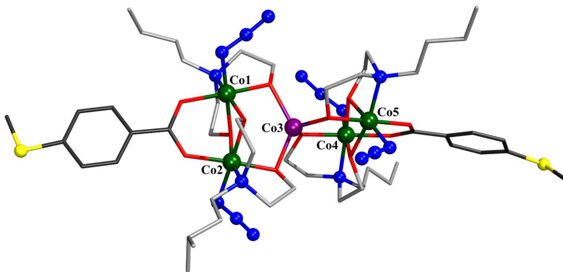
FIGURE 1 | Molecular structure of [\text{Co}^{\text{I}}\text{Co}^{\text{III}}(\text{N}_3)_4(\text{N-n-bda})_4(\text{bza-SMe})_2] ( 1 ). Hydrogen atoms and co-crystallized water molecule are omitted for clarity. The cobalt, sulfur, and the nitrogen atoms of azide groups are represented as ball-and-stick models. Color code: C (bza-SMe - ) = dark gray; C (N-n-bda 2- ) = gray; N = blue; O = red; S = yellow; Co I = violet, Co III = dark green. See Supporting Information for detailed crystal packing of the complexes.
