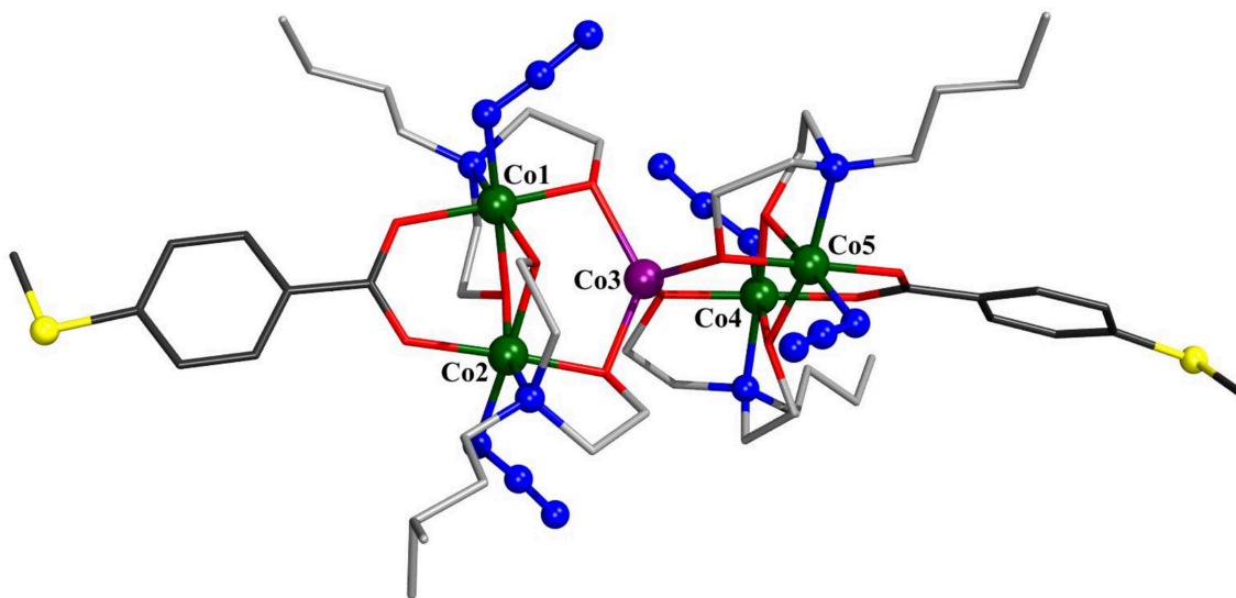
FIGURE 1 | Molecular structure of [\text{Co}^{\text{II}}\text{Co}^{\text{III}}(\text{N}_3)_4(\text{N-n-bda})_4(\text{bza-SMe})_2] ( 1 ). Hydrogen atoms and co-crystallized water molecule are omitted for clarity. The cobalt, sulfur, and the nitrogen atoms of azide groups are represented as ball-and-stick models. Color code: C (bza-SMe - ) = dark gray; C (N-n-bda 2- ) = gray; N = blue; O = red; S = yellow; Co II = violet, Co III = dark green. See Supporting Information for detailed crystal packing of the complexes.
