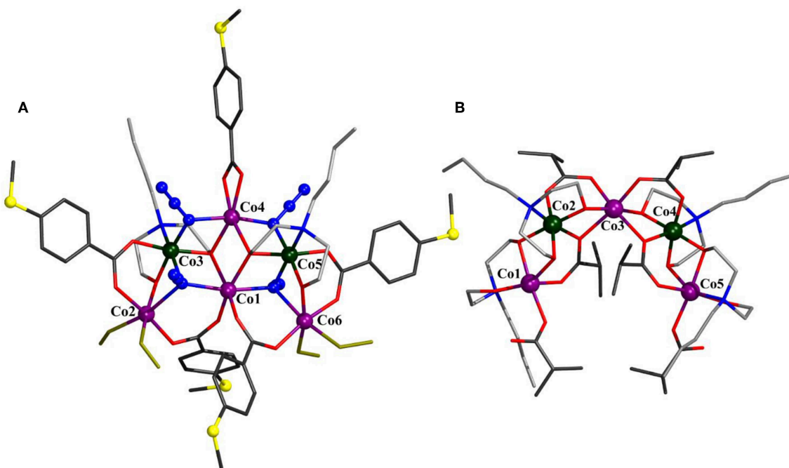
FIGURE 2 | Molecular structure of [\text{Co}_4^{\text{II}}\text{Co}_2^{\text{III}}(\text{N}_3)_4(\text{N-n-bda})_2(\text{bza-SMe})_5(\text{MeOH})_4]^+ in 2 ( A ) and comparison to [\text{Co}_3^{\text{II}}\text{Co}_2^{\text{III}}(\text{N-n-bda})_2(\text{N-n-Hbda})_2(\text{b})_6] (Schmitz et al., 2016a) ( B ). Hydrogen atoms, Cl - counterion, and co-crystallized solvent molecules are omitted for clarity. The cobalt, sulfur, and the nitrogen atoms of azides are represented as ball-and-stick models. Color code: C (carboxylates) = dark gray; C (N-n-Hbda - and N-n-bda 2- ) = gray; N = blue; O = red; S = yellow; coordinated MeOH molecules = yellow sticks; Co II = violet; Co III = dark green. See Supporting Information for detailed crystal packing of the complexes.
