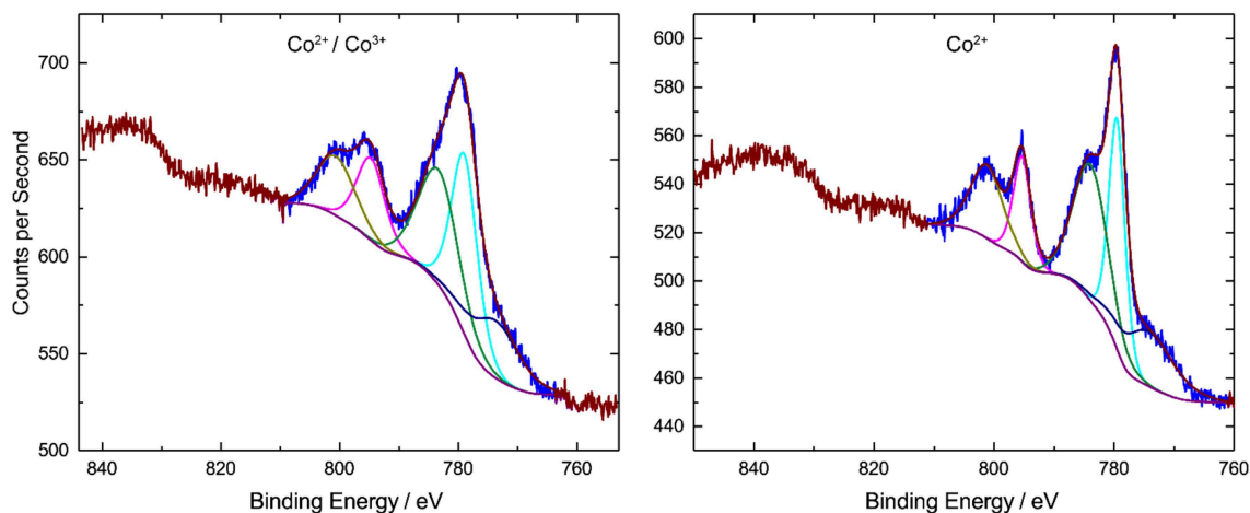
FIGURE 5 | XPS spectra of compounds 1 (left) and 1-A (right) measured in the solid state. Compound 1 features the central, high-spin Co(II) ion and the peripheral, low-spin Co(III) ions. In compound 1-A , the portion of high-spin Co(II) ions is however significantly increased.
