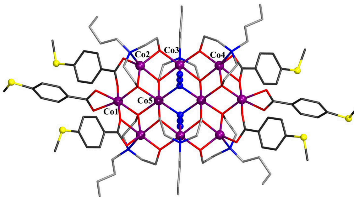
FIGURE 3 | Molecular structure of [\text{Co}_{10}(\text{N}_3)_2(\text{N-n-bda})_6(\text{bza-SMe})_6] ( 3 ) with Co numbering scheme for one asymmetric unit. Hydrogen atoms are omitted for clarity. The cobalt, sulfur, and the nitrogen atoms of azides are represented as ball-and-stick models. Color code: C (carboxylates) = dark gray; C ( N-n-bda ^{2-} ) = gray; N = blue; O = red; S = yellow; \text{Co}^{\text{II}} = violet. See Supporting Information for detailed crystal packing of the complexes.
