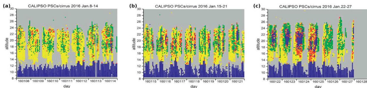
FIG. 5. Cloud occurrence for three weeks in January 2016. Vertical bars represent the altitude extent of cirrus (blue lower altitudes) and PSCs (color coded by composition: green, STS; yellow–red, mixed; blue in stratosphere, ice) observed by CALIOP along each of the ~15 orbits per day. PSCs frequently extended in altitude from the tropopause to 25-km altitude, which is more typical of the Antarctic than the Arctic. Ice clouds (blue colors) are found frequently between 20 and 25 Jan 2016.
