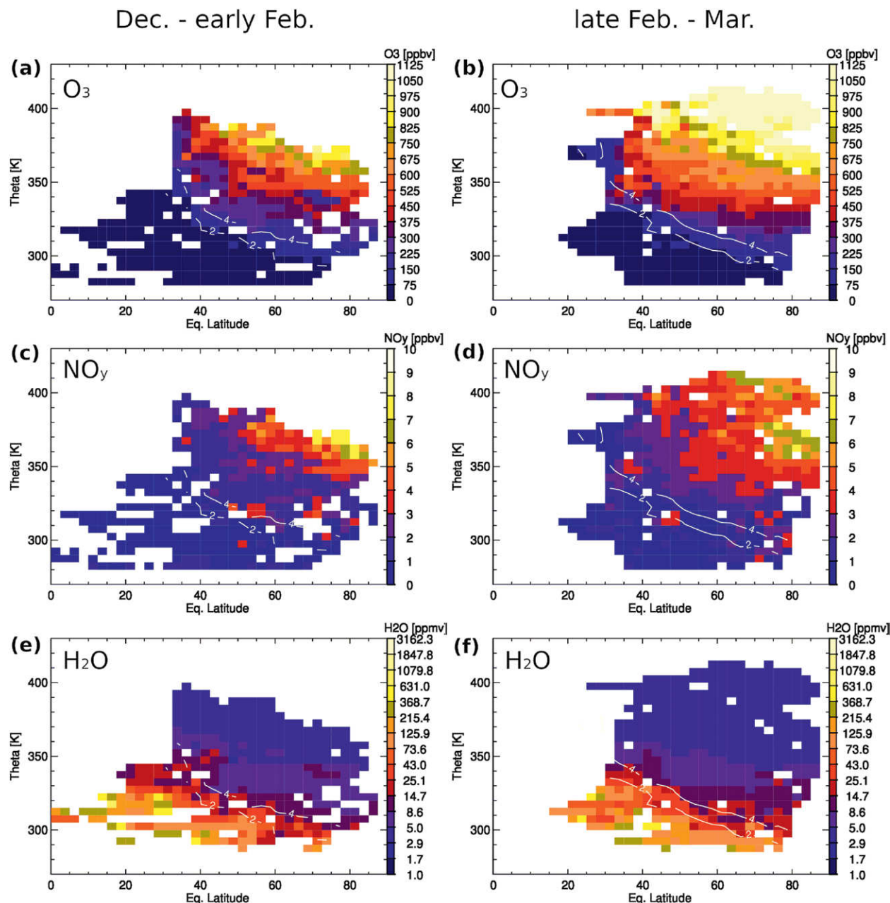
FIG. 9. As in Fig. 8, but for (top) ozone, (middle) \text{NO}_y , and (bottom) water vapor. Adapted from Krause et al. (2018).
