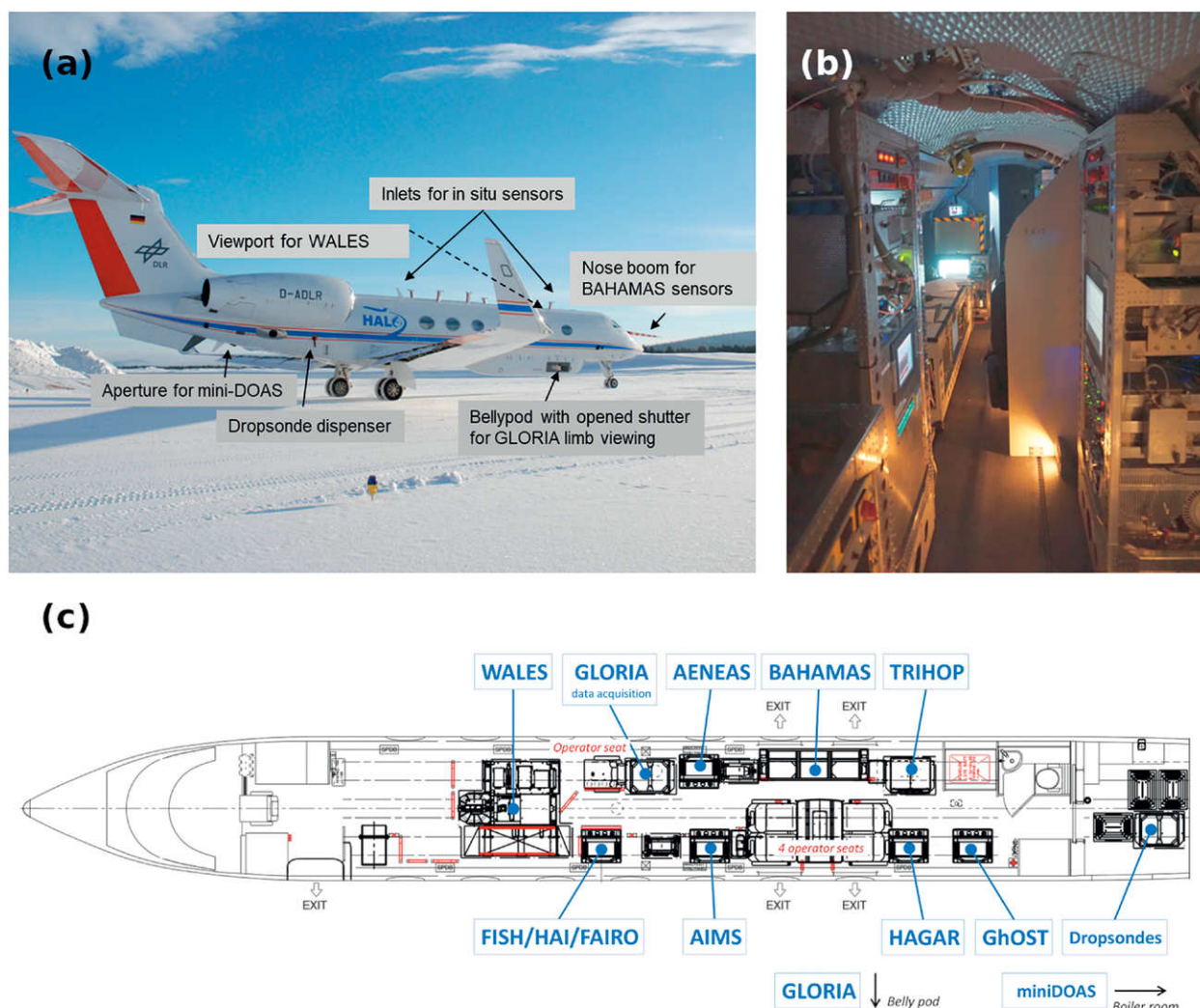
FIG. 2. (a) HALO in POLSTRACC configuration, (b) cabin view with POLSTRACC instrumentation, and (c) corresponding cabin layout.
