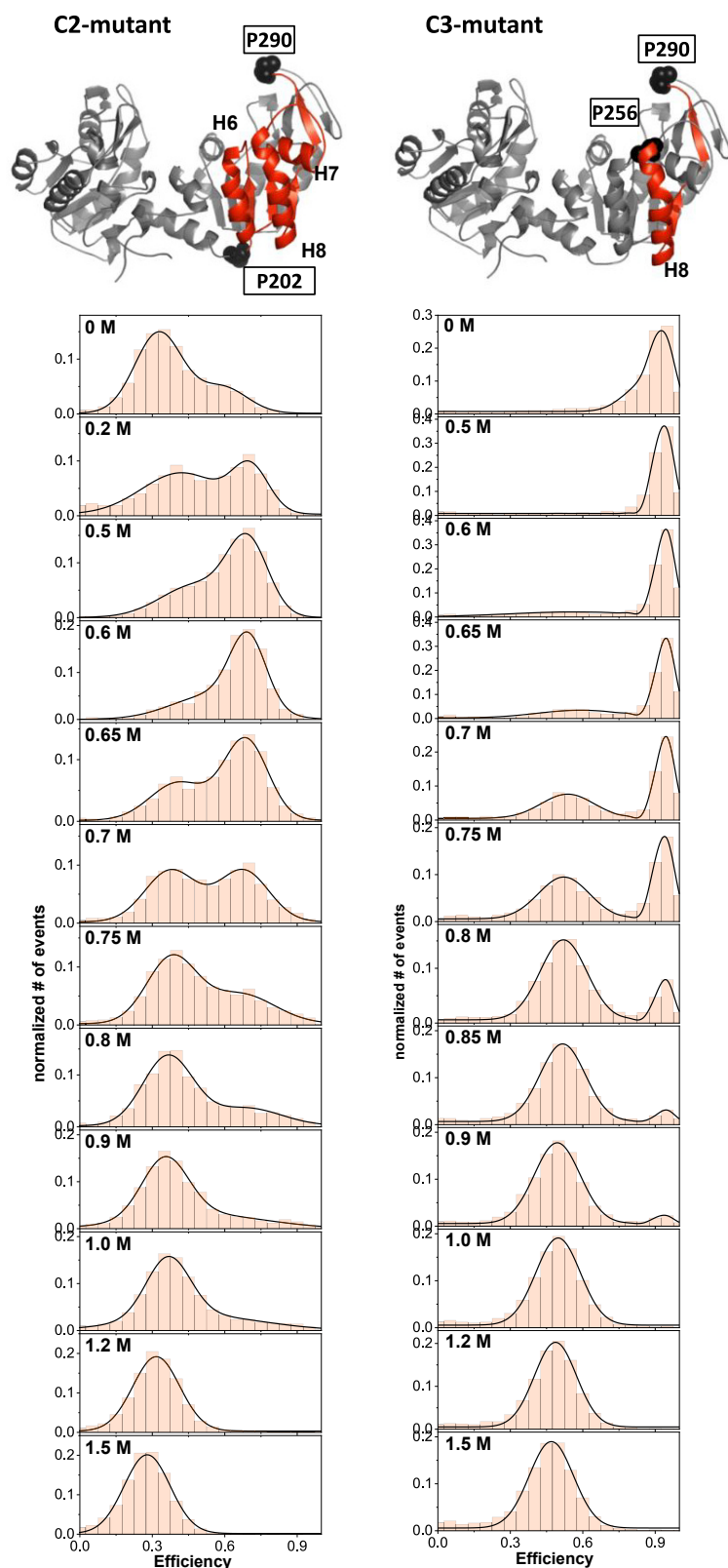
FIGURE 3 Properties of two further intradomain distances within the C-domain. The interdy distance of the C2 mutant is given by a measured R_{DA} = 57 \text{ \AA} , whereas that of the C3 mutant yields a measured R_{DA} = 31 \text{ \AA} . Structure elements enclosed between the dye attachment positions are highlighted in red (C2 mutant: 88 residues; C3 mutant: 34 residues) and includes C2 mutant with 4 \beta -sheets and 3 \alpha -helices and C3 mutant with 2 \beta -sheets and 1 \alpha -helix. To see this figure in color, go online.
