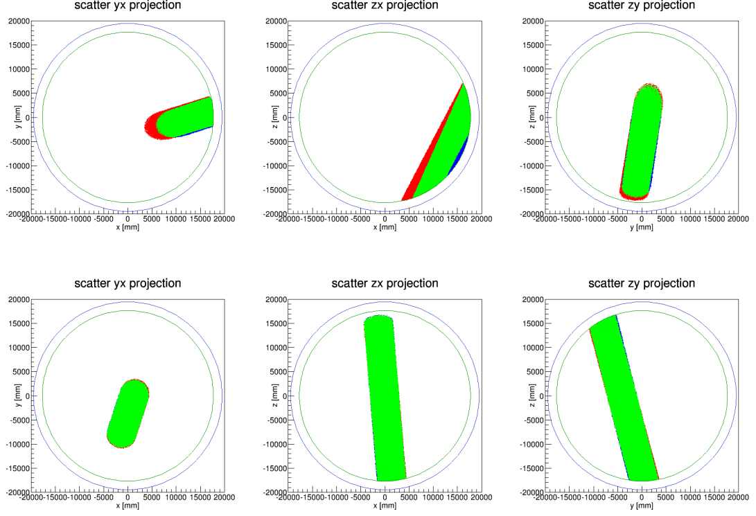
Figure 5.15 – Visualization of veto cylinders with r_v = 3\text{ m} around the true and reconstructed track. The blue area shows the projection of the cylinder around the true track, while the cylindrical volume around the reconstructed track is red. The overlap of both volumes is colored in green. In the top row three projections of a badly reconstructed track are shown and the difference between the volumes is clearly visible. The bottom row shows the same projections for a well reconstructed track, where both cylinders overlap almost completely.
