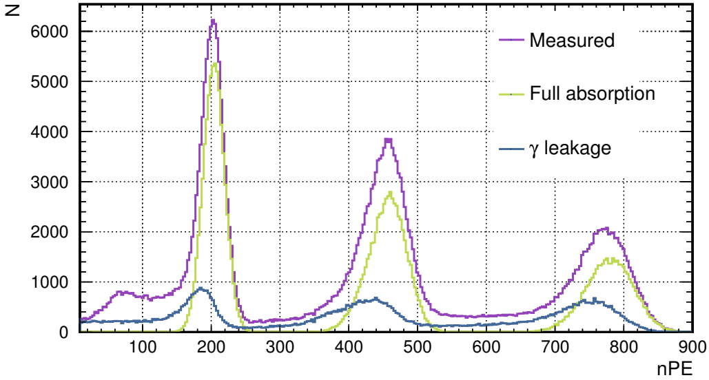
Figure 8.9 – Energy spectrum of ^{137}\text{Cs} , ^{40}\text{K} , and ^{60}\text{Co} in one capsule at \rho = 120 cm and z = 0 cm in the central detector plane. The sub-spectra of full absorption and \gamma -leakage show, that the effect is smaller in the middle of the axis in comparison to the extreme point of z = 120 cm in Figure 8.7. All three peaks are well separated and do not interfere.
