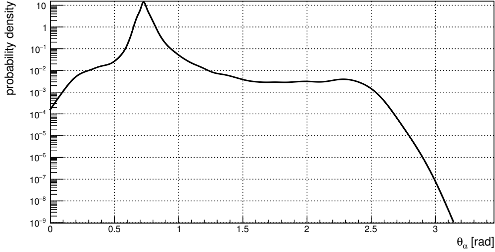
Figure 5.8 – Probability density function of \theta_\alpha for D = 0 m for the LPMT cone-part of the model. It is produced by plugging-in the first hit times from the Monte Carlo simulation of muon tracks into the reconstruction model. It was smoothed over the whole domain of definition with adaptive kernel density estimators [118].
