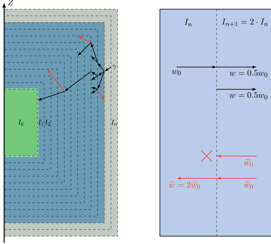
Figure 6.5 – Left: Principal visualization of the parallel geometry implemented in the detector simulation. The LS target is assigned the largest importance value I_0 = \alpha^{N_s} , while the outward going shells follow I_i = \alpha^{N_s-i} for their importance value. An exemplary \gamma -track starting in the rock is shown. Black tracks move towards a higher importance shell, while red tracks enter a shell with lower importance. Right: Working principle of the splitting and killing of tracks in the biasing algorithm for an importance ratio r = I_{n+1}/I_n = 2 .
