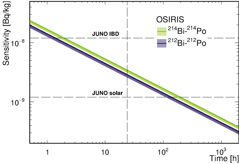
Figure 7.8 – Sensitivity of OSIRIS as a function of the measurement time for the ^{212}\text{Bi} - ^{212}\text{Po} (purple) and ^{214}\text{Bi} - ^{214}\text{Po} (green) coincidence searches. The sensitivity is given as a 90% CL upper limit on the contamination. While the line at the upper end of the band gives the sensitivity with maximal estimated Radon contamination, the band shows the improvement of the sensitivity up to no additional Radon contamination in the water shield. Within a few hours, OSIRIS can verify the JUNO IBD requirement. In order to confirm a contamination of 1 \times 10^{-9} \text{Bq/kg} required for solar neutrinos, a measurement longer than one day is needed.
