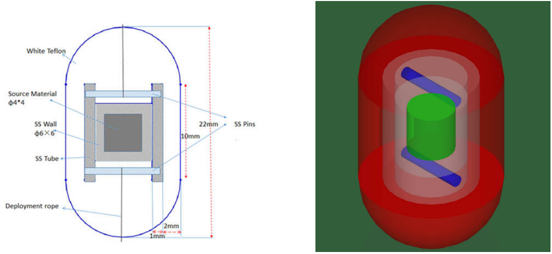
Figure 8.3 – Left: Technical drawing of a calibration capsule prototype for JUNO (internal design by collaboration). Right: Visualization of the implemented geometry in the OSIRIS simulation.
