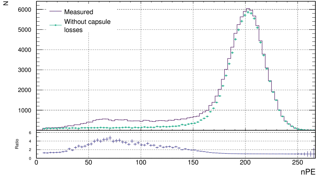
Figure 8.8 – Histogram of the measurable nPE spectrum of ^{137}\text{Cs} at \rho = 120 cm and z = 0 cm. The overlaid points with error bars show the corresponding spectrum of all events except those with energy losses in the capsule. At the bottom the ratio of both spectra is plotted. It shows, that the peak region is not affected by losses in the capsule.
