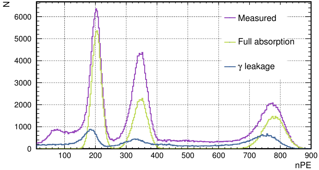
Figure 8.10 – Energy spectrum of ^{137}\text{Cs} , ^{65}\text{Zn} , and ^{60}\text{Co} in one capsule at \rho = 120 cm and z = 0 cm in the central detector plane. Although the ^{65}\text{Zn} peak is closer to the one of ^{137}\text{Cs} , they are still sufficiently separated.
