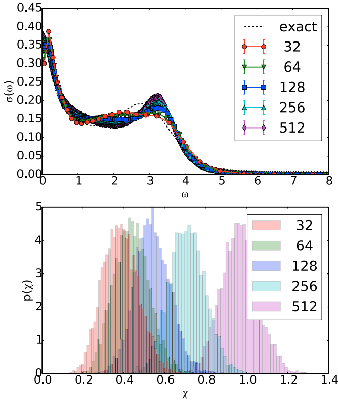
FIG. 8. Dependence of the average spectrum on the number N of grid points for the same problem as in Fig. 7 on a Lorentzian with \gamma = 2.5 . For larger N , the average spectra get worse. The reason becomes clear from the histograms in the bottom panel, showing the contribution of spectra with a given fit \chi to \tilde{\mathbf{f}}_{\text{ASM}} : with increasing N the histogram moves to the right, i.e., worse fits.
