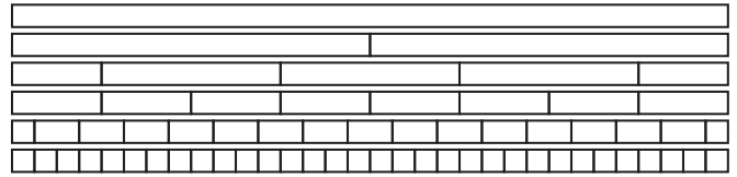
FIG. 2. Example of the hierarchy of grid partitionings used in blocked-mode sampling. At the highest level (top), the grid on which \mathbf{f} is represented forms a single block. Sampling on this block is modes sampling. At the level below, the grid is split into two blocks. If going to a lower level we split the blocks in half, there would always be a block boundary at the center of the grid. To avoid this, we shift the intervals at every other level by half their width. At the lowest level (bottom), the blocks are the individual intervals f_n . Sampling on these blocks is components sampling.
