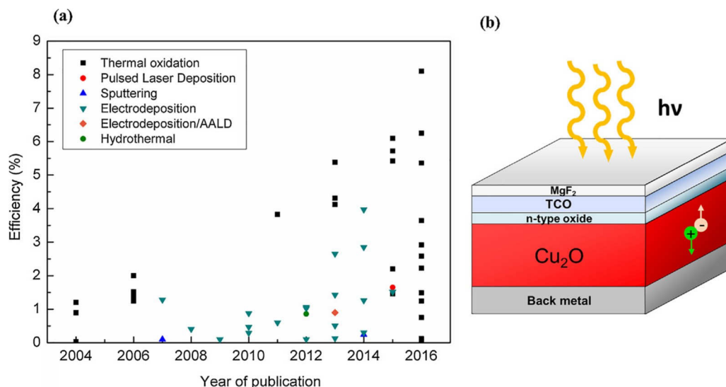
Fig. 47. (a) Plot showing all-oxide \text{Cu}_2\text{O} -based solar cells reported efficiencies by different deposition techniques for the \text{Cu}_2\text{O} layer. (b) Scheme of a typical \text{Cu}_2\text{O} -based solar cell.
