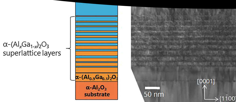
Fig. 59. Cross-sectional TEM image of \alpha -Ga 2 O 3 on sapphire with quasi-alloy buffer layers [910].
