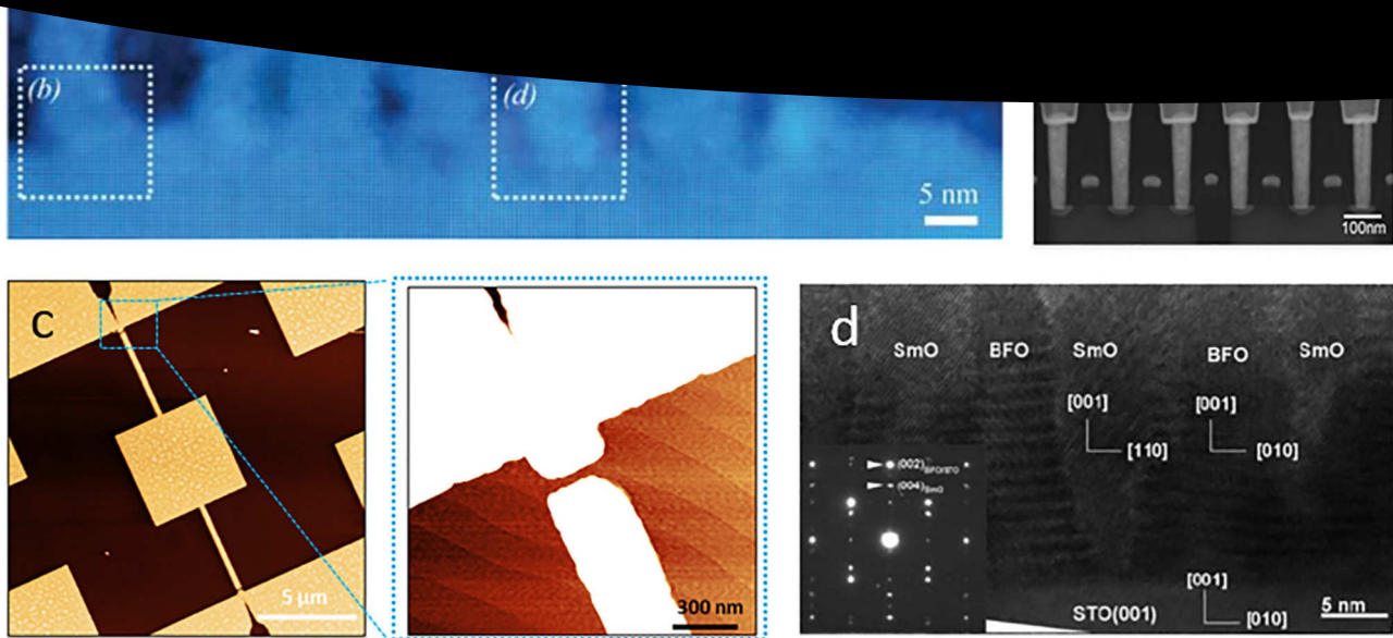
Fig. 12. Examples of nanoscale oxide structures. (a) Crystalline oxide sculpting using scanning transmission electron microscope (STEM): Fourier-filtered HAADF image of the arbitrary graphical pattern created in the amorphous region of \text{SrTiO}_3 . Copyright [2015] Wiley-VCH Verlag GmbH & Co. KGaA, Weinheim. Reprinted with permission from [105]. (b) A 40-nm \text{Ir(TE)/Ta}_2\text{O}_5/\text{TaO}_x/\text{TaN} (BE) RRAM memory [106]. (c) Superconducting quantum interference device based on nano-constrictions [107]. Note the side gates to control the transport through the constrictions. (Figure courtesy of A. Caviglia) (d) Cross-sectional TEM images of a (\text{BFO})_{0.5}:(\text{SmO})_{0.5} VAN thin film. Copyright [2010] IOP Publishing Ltd. Reprinted with permission from [108].
