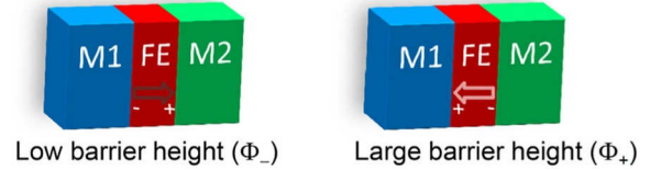
Fig. 23. Tunnel electroresistance induced by the modulation of the potential profile of the ferroelectric (FE) barrier when polarization is reversed in the case of electrodes (M1 and M2) with different effective screening lengths ( \delta_1 and \delta_2 ). The average barrier height is lower, \Phi_- (higher, \Phi_+ ) when the polarization points toward M2 (M1), resulting in the ON (OFF) state resistance. Adapted from [306].
