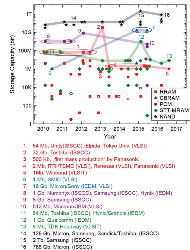
Fig. 21. Evolution of the storage density of different types of emerging memories in comparison with ReRAM. (Extracted with permission from [295]).
