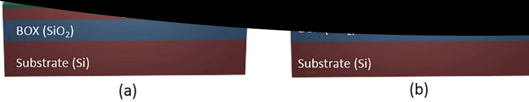
Fig. 40. Examples of Si-compatible (a) BaTiO 3 and (b) VO 2 waveguides.
