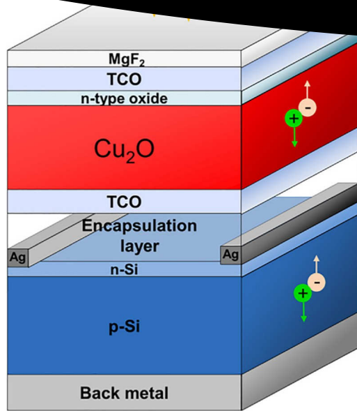
Fig. 48. Scheme of a \text{Cu}_2\text{O} -Si-based tandem solar cell.
