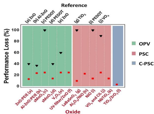
Fig. 46. Performance loss after stability analysis, for solar cells applying oxides as transport layers (red squares) and the corresponding reference solar cell (black triangles) for organic solar cells (OPVs), perovskite solar cells (PSCs) and carbon-based PSCs (C-PSCs). The solar cell configuration and the stability analysis conditions are: Organic solar cells (OPV): (a) ITO/ZnO:PEIE/P3HT:PCBM/MoO 3 /Ag and ITO/ZnO/P3HT:PCBM/MoO 3 /Ag [666]. (b) ITO/Al-ZnO:PEIE/P3HT:PCBM/MoO 3 /Ag and ITO/Al-ZnO/P3HT:PCBM/MoO 3 /Ag [666]. (c-d) ITO/MoO 3 /P3HT:PCBM/Al:Ag and ITO/PEDOT/P3HT:PCBM/Al:Ag in Air (c) and in N 2 (d) [667]. (e) FTO/V 2 O 5 /P3HT:PCBM/ZnO/Ag and FTO/ZnO/P3HT:PCBM/V 2 O 5 /Ag [668] and (f) UV Filter/FTO/ZnO/P3HT:PCBM/V 2 O 5 /Ag [668]. (g) FTO/LaBaSnO 3 /MAPbI 3 /PTAA/Au and FTO/TiO 2 /MAPbI 3 /PTAA/Au. Photostability tests under constant AM 1.5G illumination with a xenon lamp, including UV radiation [663] (h) FTO/TiO 2 /mp-TiO 2 /Al 2 O 3 /NiO/MAPbI 3 -xCl x -NiO/Spiro-OMeTAD/Au [669]. (i) ITO/NiOx/Perovskite/ZnO/Al and ITO/PEDOT:PSS/Perovskite/PCBM/AL [670]. (j) ITO/PEDOT:PSS/VO x /Perovskite/PCBM/CIL/Ag and ITO/PEDOT:PSS/VO x /Perovskite/PCBM/Ag. 200 h in ambient conditions without any encapsulation. [671]. (k) FTO/NiMgLiO/MAPI/PCBM/NbTiO x /Ag [672]. (l) FTO/TiO 2 /ZrO 2 /Carbon + 2D:3D Perovskite. 10000 h [673]. Tables and detailed information can be found in [665]. (For interpretation of the references to color in this figure legend, the reader is referred to the web version of this article.)
