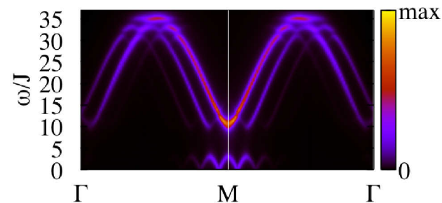
Figure 7.3.4: Total spin-wave scattering spectrum for the Mn/ \beta -W. The figure shows the dispersion curves of the rotational and longitudinal helimagnon modes on a reciprocal path along q . The gap of about 5 meV in the spectrum is due to the magnetocrystalline anisotropy. Below the gap, the minima at \pm q of the rotational modes can be observed. Above, the central and brightest feature is composed of the longitudinal and rotational modes.
