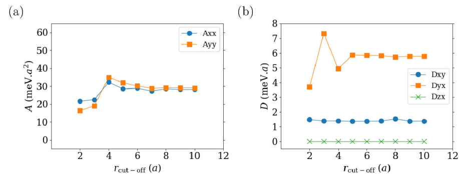
Figure 8.B.4: Estimate of the stiffness and spiralization-tensor elements as a function of the cut-off radius, using the extrapolation method, for the pseudomorphic 1ML Co/W(110). (a) shows the convergence of the stiffness-tensor elements and (b) represents the spiralization-tensor elements. These values converge much quicker than those obtained through direct summation shown in Figs. 8.4.1 and 8.4.2.
