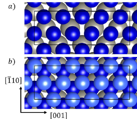
Figure 5.3.1: (a) Top view of a Co ML on W(110), in the 4 \times 1 reconstruction. The dark blue spheres represent Co atoms, while the gray ones are W atoms. The crystallographic directions for bulk W are also indicated. Five Co atoms are covering four W atoms in the [001] direction. (b) 2ML Co on W(110) in hcp stacking. The Co layer at the interface is shown with dark blue spheres, while light blue spheres depicting the second Co layer.
