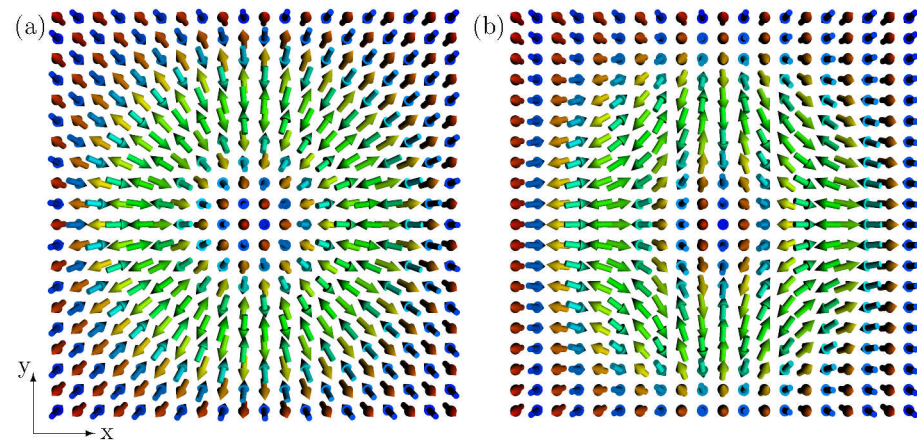
Figure 7.2.4: Skyrmion-like structures in an antiferromagnetic background. (a) Antiferromagnetic skyrmion that is formed when the exchange interaction with all nearest neighbors is negative, Model I. The skyrmion lies in a c(2 \times 2) antiferromagnetic background. (b) Antiferromagnetic antiskyrmion, which results from anisotropy exchange interactions. J is negative along- x and positive along- y , Model II. The antiskyrmion lies in a p(2 \times 1) antiferromagnetic background. Model parameters: |J| = 1 , D = 0.2 , K = 0.05 and B = 0 a.u. The total energy of both spin configuration is E = -4.041052J .
