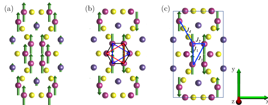
Figure 7.4.1: Different self-consistent magnetic phases. (a) FM: Ferromagnetic phases obtained by spin polarizing the system with a magnetic field during the first self-consistent interaction of the Kohn-Sham cycle. The magnetic moments are of 2.6 and 1.1 \mu_B . (b) AFM: The antiferromagnetic phase obtained self-consistently after reversing the magnetic moment orientation of some sites of the ferromagnetic phase. The magnetic moments are of 2.4 \mu_B . The AFM phase is energetically more favorable than the FM one. (c) Indication of the first few exchange interaction pairs. Atoms connected by the red triangle in (b) are in the same plane, and atoms linked by the blue triangle are in another plane. From this top view, the two triangles together form a hexagon.
