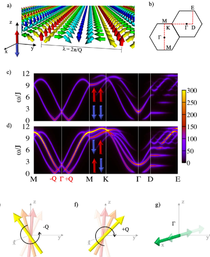
Figure 6.3.2: Spin-waves for a spin-spiral structure, beam polarization along z . (a) Spin-spiral ground state and crystallographic axes. The red and blue arrows correspond to the two considered spin polarizations of the electron beam. (b) Path in reciprocal space being considered for the calculations of the SREELS spectra. These are shown in (c) for the spin-conserving channels, and in (d) for the spin-flip channels. The arrow pairs indicate the initial and final electron spin polarization for each channel. (e-g) Sketch of the low-frequency motion of the net atomic spin for the three spin-wave modes with minima in -Q , +Q and \Gamma , respectively.
