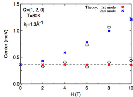
Figure 7.4.3: Spin-wave dispersion at \mathbf{q} = (1, 2, 0) as a function of the external magnetic field (crosses) in comparison to the energy center of the experimental inelastic-neutron-scattering data (open circles) [153]. The magnetic exchange and magnetic anisotropy parameters were rescaled by a factor of 10 to reproduce the experimental energy gap.
