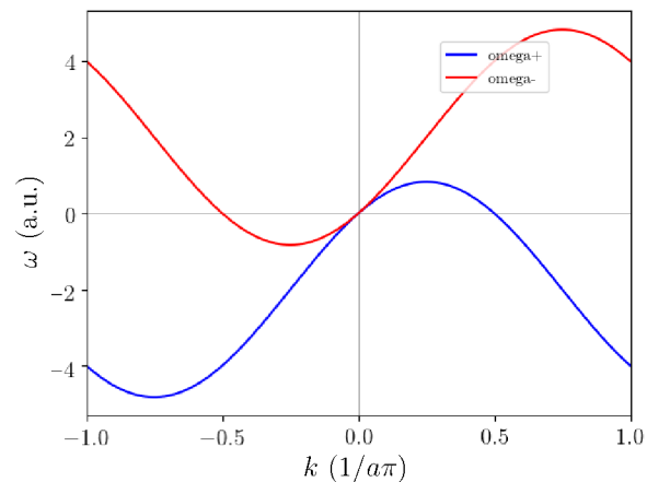
Figure 9.A.1: Spin-wave dispersion for a ferromagnet with DMI. The red and blue curves correspond to the values \omega^- and \omega^+ , respectively. The negative part of \omega^- indicates an instability of the ferromagnetic spin configuration: with the DMI, the ground state passes to be a spin spiral. The blue curve is obtained from the red one by reversing the space and time, which take k \rightarrow -k and \omega^+ \rightarrow -\omega^- .
