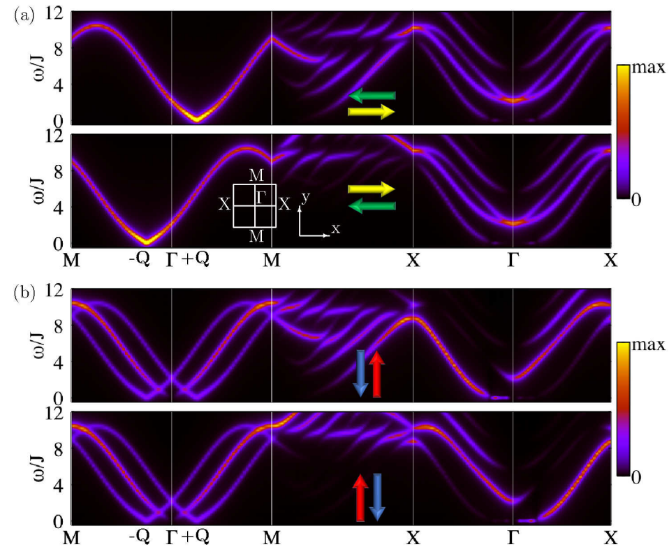
Figure 9.3.4: Spin-resolved inelastic-scattering spectra for the spin spiral generated by Model I. (a) Shows the two spin-flip channels for polarization along \hat{\mathbf{x}} , as indicated by the horizontal arrows. Nonreciprocity occurs in the reciprocal space where a component of \mathbf{D}(\mathbf{k}) , polarization and angular momentum align with each other. For Model I on path M- \Gamma -M, \mathbf{D}(\mathbf{k}) and the angular momentum of the spin-wave modes with minima at \mathbf{k} = \pm\mathbf{Q} are parallel to \hat{\mathbf{x}} . (b) Shows the case for the polarization along \hat{\mathbf{y}} , indicated by the vertical arrows. Thus, nonreciprocity is only seen in the X- \Gamma -X, when \mathbf{D}(\mathbf{k}) \parallel \hat{\mathbf{y}} that couples to the angular momentum of those spin waves.
