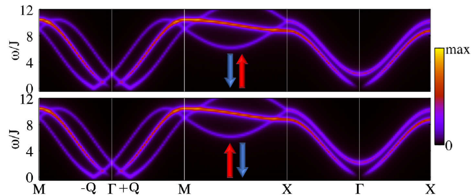
Figure 9.3.8: Spin-resolved inelastic-scattering spectra for the spin spiral generated by Model I with D^y = 0 . Note that the spiral itself is stabilized by D_x . The polarization is set along \hat{\mathbf{y}} , as indicated by the vertical arrows. The two spin-flip channels are degenerate and reciprocal because \mathbf{D}(\mathbf{k}) has no component along the polarization to induce angular momentum of the spin-wave modes along that direction. Restoring the D^y of the original Model I, a nonreciprocity occurs on the X- \Gamma -X while the ground-state spin configuration is not affected, proving that the DMI can directly induce the nonreciprocity of spin waves.
