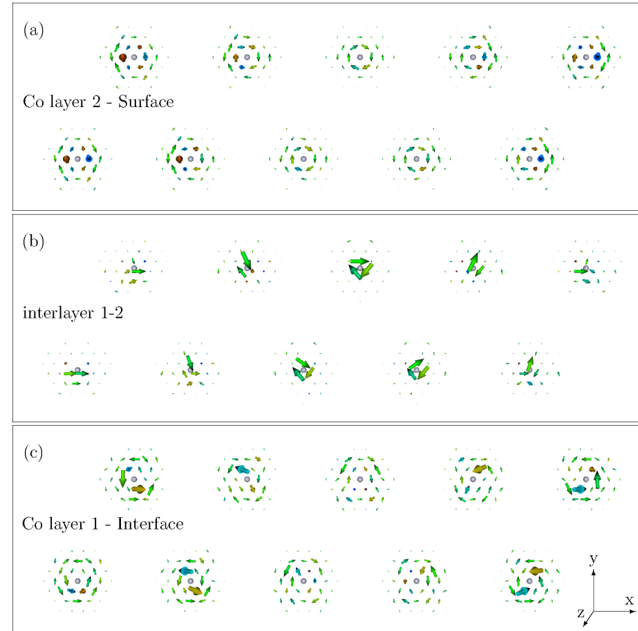
Figure 8.3.3: Dzyaloshinskii-Moriya vectors for the 2 MLs reconstructed cobalt film. (a) and (c) show the intralayer interactions of the film surface and interface, respectively. (b) displays the interlayer DMI interactions between the two cobalt layers. Each cluster of vectors represent the interactions of one atom in the unit cell (the gray sphere) and its neighbors. The centers of the vectors are located on the position of the neighbors. The color code paints in blue and red out-of-plane vectors, and green the in-plane ones. The biggest arrow corresponds to a DMI strength of 0.63 meV. The interface with the substrate makes every cluster different from the others. Out-of-plane components are mostly observed on the nearest-neighbor couplings at the surface.
