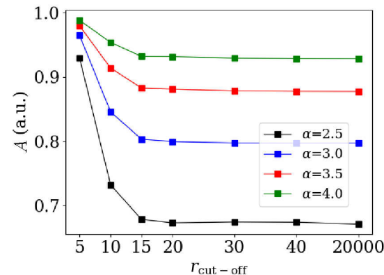
Figure 8.B.3: Stiffness constant estimate as a function of the cut-off radius for different power-law coefficients \alpha . The estimates were obtained via the extrapolation methods discussed in the text. The last point of all curves corresponds to the exact numerical solution. A cut-off radius equal or bigger to 20 seems to yield a good estimate of A . For a smaller radius, we can observe discrepancies from the exact solution, which are bigger the smaller \alpha is. Parameters: a = 1 , \lambda = 4a .
