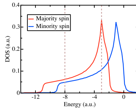
Figure 5.3.7: Total density of states of the two-band model given in Eq. (5.7). The dashed lines mark a Fermi energy near the bottom of the two bands (left), and another at the Van Hove singularity (right). The correspondent Fermi surface is almost isotropic in the first case, and very anisotropic in the other; see Fig. 5.3.8. t = -1 , U = 1 , E_0 = -4 , and \eta = 0.1 a.u.
