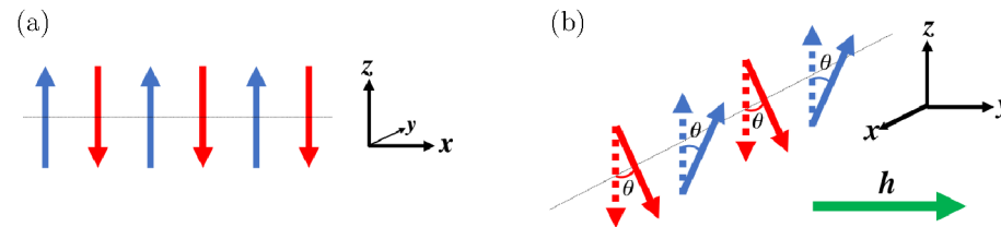
Figure 7.4.4: Unidimensional spin chain. (a) With J < 0 , we obtain an antiferromagnetic spin alignment. (b) When an external magnetic field is applied \mathbf{h} , the spin moments tilt away from the equilibrium by an angle \theta .
