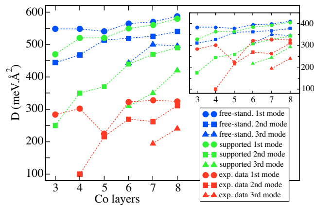
Figure 5.4.2: Stiffness constants obtained from fitting the spin-wave branches of Fig. 5.4.4 to Eq. (5.13). Blue refers to the free-standing calculations while green stands for the supported case. Red indicates the stiffness of the experimental data [24]. For all fits, only points with q_{\parallel} < 0.3 \text{ \AA}^{-1} were considered. Circles correspond to the first (acoustic) mode, squares to the second mode, and triangles to the third one. The inset presents the same data as above with free-standing and supported results rescaled down by 30%, as will be discussed in Sec. 5.4.2. The supported films capture the experimental trends better than the free-standing ones.
