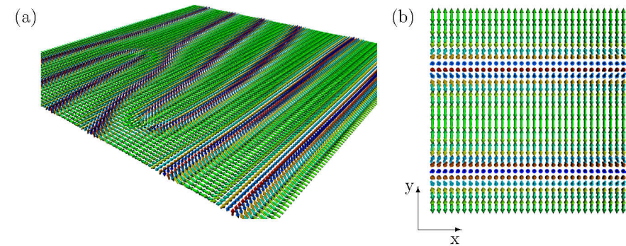
Figure 7.3.3: The ground-state magnetic structure of the Mn monolayer on \beta -tungsten. (a) A 100 \times 100 super cell with periodic boundary conditions was considered for a spin-relaxation dynamics starting from a random configuration. From this simulation, an antiferromagnetic spin-spiral pitch of 32 atomics distances could be estimated. (b) A 32 \times 32 supercell was considered to obtain the ground-state spin configuration of the Mn/ \beta -W. We used an easy-axis anisotropy along y with K = 1.5 meV.
