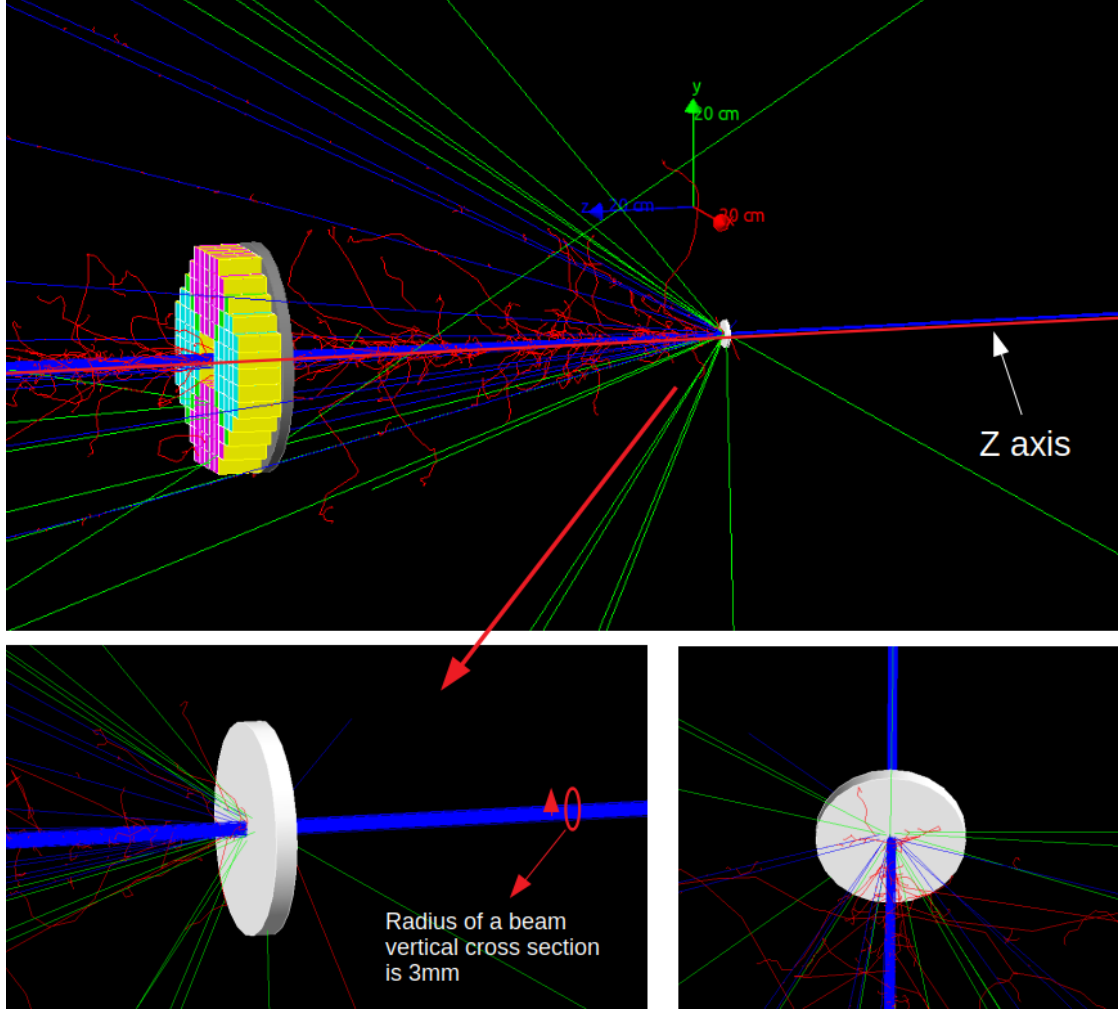
Figure 3.6: Particle generator geometry in GEANT4 model of 2017.
