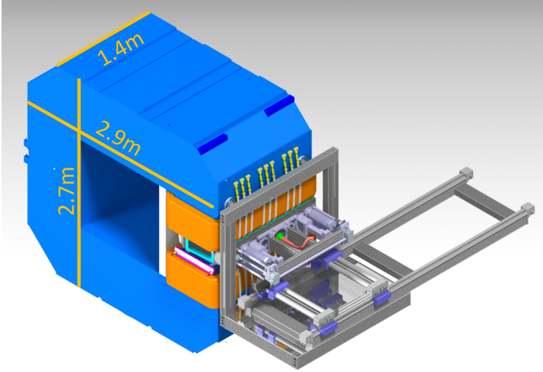
Figure 31: CAD drawing of the large setup inside the magnet with the support structure at the front [34].
