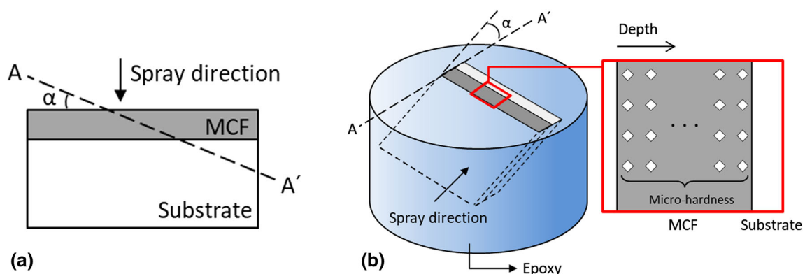
Fig. 1 Schematic view of the (a) cross section and (b) location used for micro-hardness testing on the oblique section
