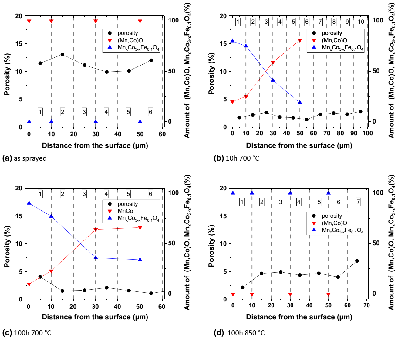
Fig. 3 Porosity depth distribution and depth distribution of the volume fraction of salt rock and spinel structure within the MCF coating for different annealing treatments
