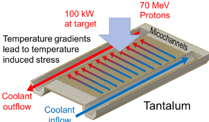
Figure 7: Target design for a large scale facility source at a power level of 100 kW.
