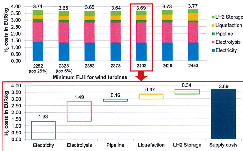
Figure 2. Cost distribution over all elements of the hydrogen supply chain for the considered degrees of expansion of wind energy in Saudi Arabia.
