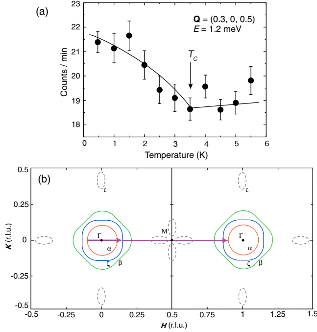
FIG. 4. (a) Temperature dependence of the scattering intensity at \mathbf{Q} = (0.3, 0, 0.5) with E = 1.2 meV, which clearly shows a kink at T_c . The data show clearly order-parameter-like increase below T_c , a hallmark of the neutron spin resonance. The solid line is a guide to the eyes. (b) Schematic of the hole Fermi pockets in \text{KFe}_2\text{As}_2 in the Brillouin zone, inferred from de Haas–van Alphen and ARPES measurements [17,27,28]. The purple arrows indicate the interband scattering.
