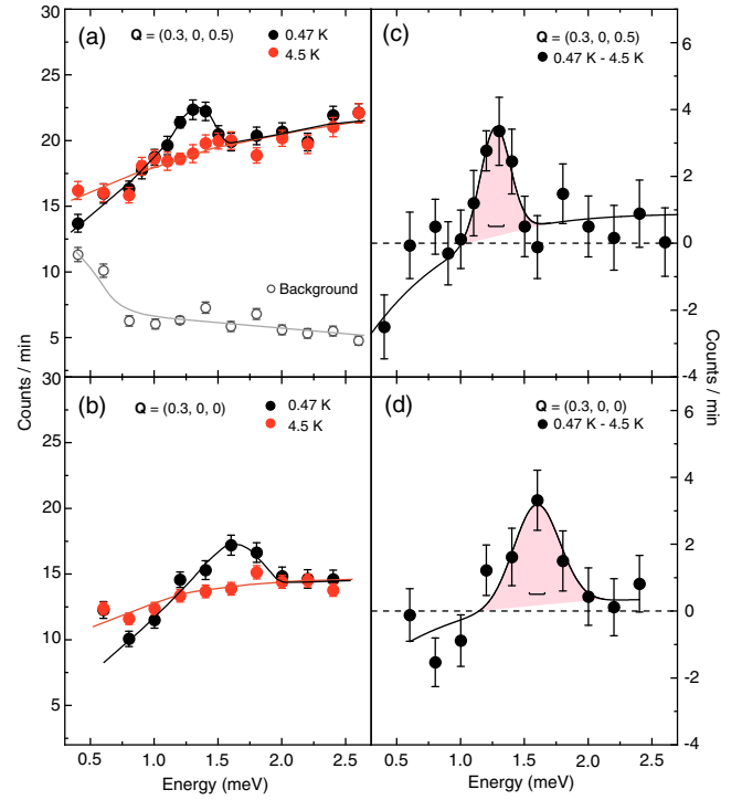
FIG. 3. Energy dependence of spin excitations for \text{KFe}_2\text{As}_2 . (a), (b) Constant- \mathbf{Q} scans in the superconducting state ( T = 0.47 K) and normal state ( T = 4.5 K) for \mathbf{Q} = (0.3, 0, 0.5) and \mathbf{Q} = (0.3, 0, 0) , respectively. For comparison, the background scattering measured at \mathbf{Q} = (0.2, 0, 0.5) and (0.5, 0, 0.5) is also shown. (c),(d) Temperature difference plot shows clear spin resonance at E = 1.2 meV for \mathbf{Q} = (0.3, 0, 0.5) and E = 1.6 meV for \mathbf{Q} = (0.3, 0, 0) , respectively. The horizontal bars indicate the instrument resolution ( \sim 0.12 meV). The FWHM of the resonance peaks at L = 0.5 and L = 0 are \sim 0.27 and \sim 0.51 meV, respectively.
