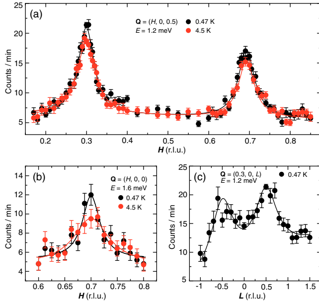
FIG. 2. Momentum dependence of the magnetic excitations. (a),(b) Constant energy scans below and above T_c at E = 1.2 meV along (H, 0, 0.5) direction and at E = 1.6 meV along (H, 0, 0) direction, respectively. (c) Constant energy scan along the (0.3, 0, L) direction at E = 1.2 meV below T_c . The spin fluctuations exhibit L modulation and are peaked at the half-integer positions. Solid lines are Lorentz fits to the data.
